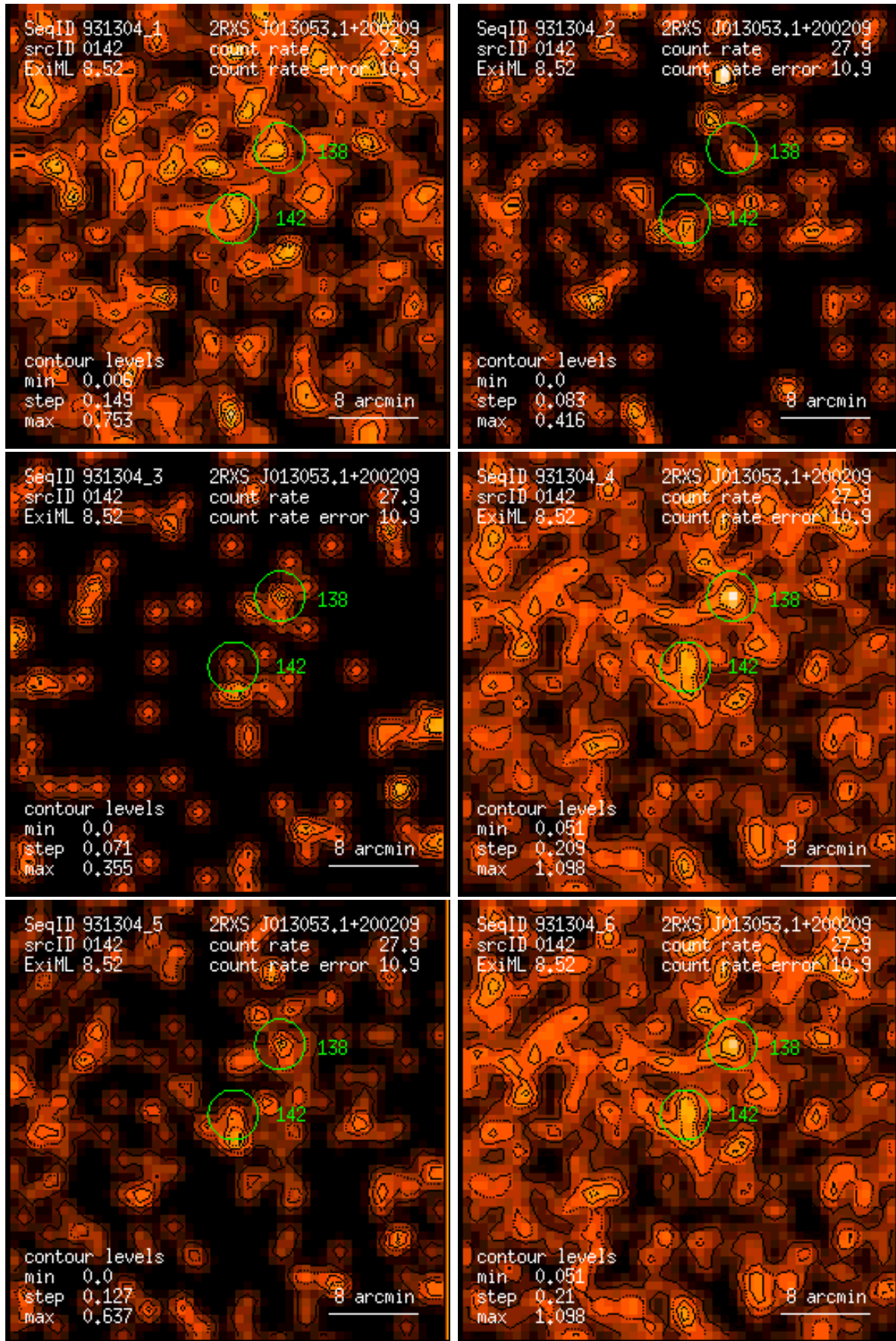
Figure 142: RASS 931304: detection 0142: band rate images, Gaussian filter: (1) PSPC channels 11 – 41, (2) 52 – 90, (3) 91 – 201, (4) 11 – 235, (5) 52 – 201, (6) 11 – 201. Broad band rates in counts/ks. Band rate contour levels in counts/ks/arcmin 2 .
