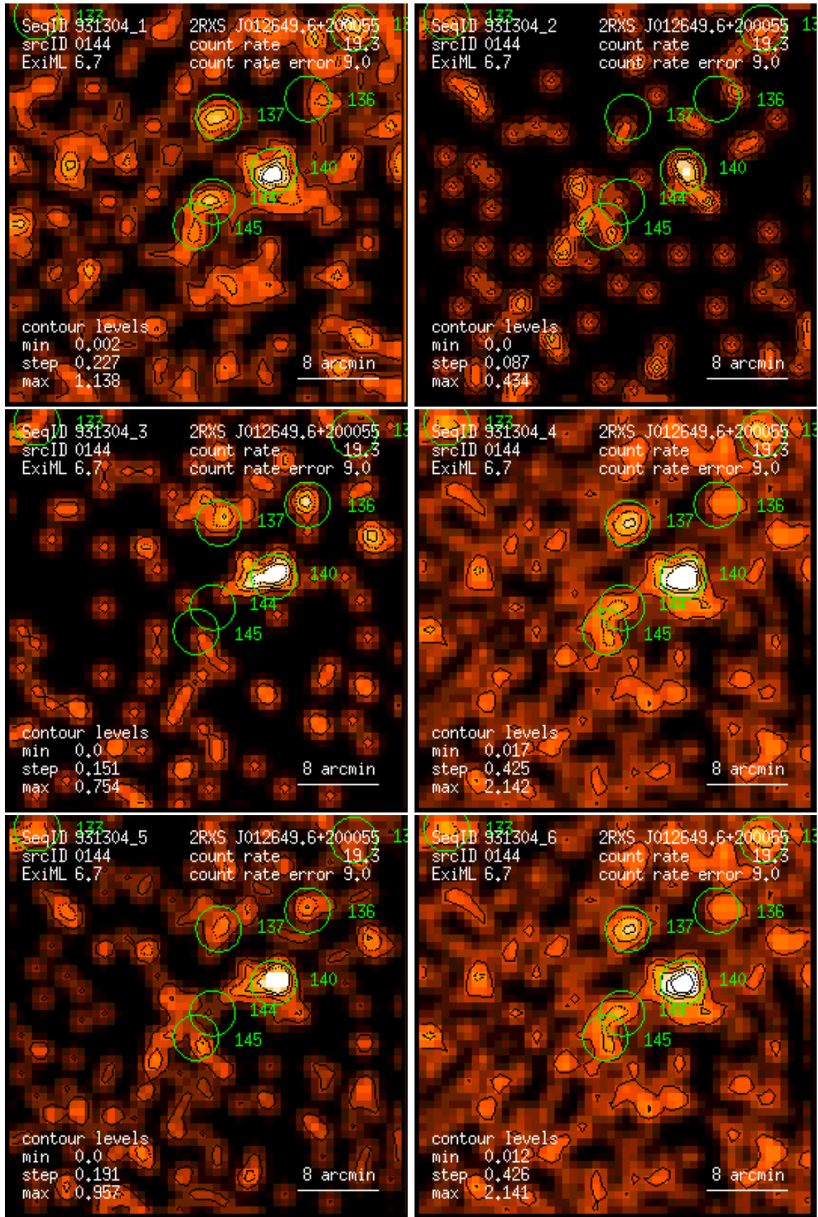
Figure 144: RASS 931304: detection 0144: band rate images, Gaussian filter: (1) PSPC channels 11 – 41, (2) 52 – 90, (3) 91 – 201, (4) 11 – 235, (5) 52 – 201, (6) 11 – 201. Broad band rates in counts/ks. Band rate contour levels in counts/ks/arcmin 2 .
