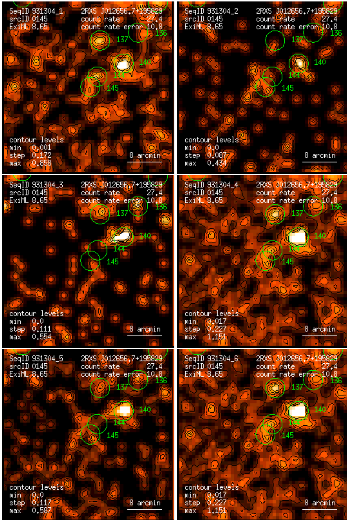
Figure 145: RASS 931304: detection 0145: band rate images, Gaussian filter: (1) PSPC channels 11 – 41, (2) 52 – 90, (3) 91 – 201, (4) 11 – 235, (5) 52 – 201, (6) 11 – 201. Broad band rates in counts/ks. Band rate contour levels in counts/ks/arcmin 2 .
