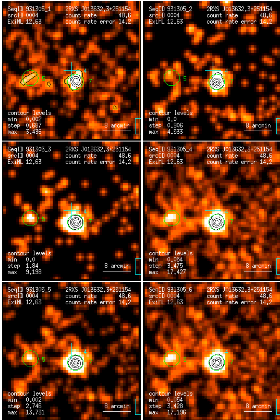
Figure 4: RASS 931305: detection 0004: band rate images, Gaussian filter: (1) PSPC channels 11 – 41, (2) 52 – 90, (3) 91 – 201, (4) 11 – 235, (5) 52 – 201, (6) 11 – 201. Broad band rates in counts/ks. Band rate contour levels in counts/ks/arcmin 2 .
