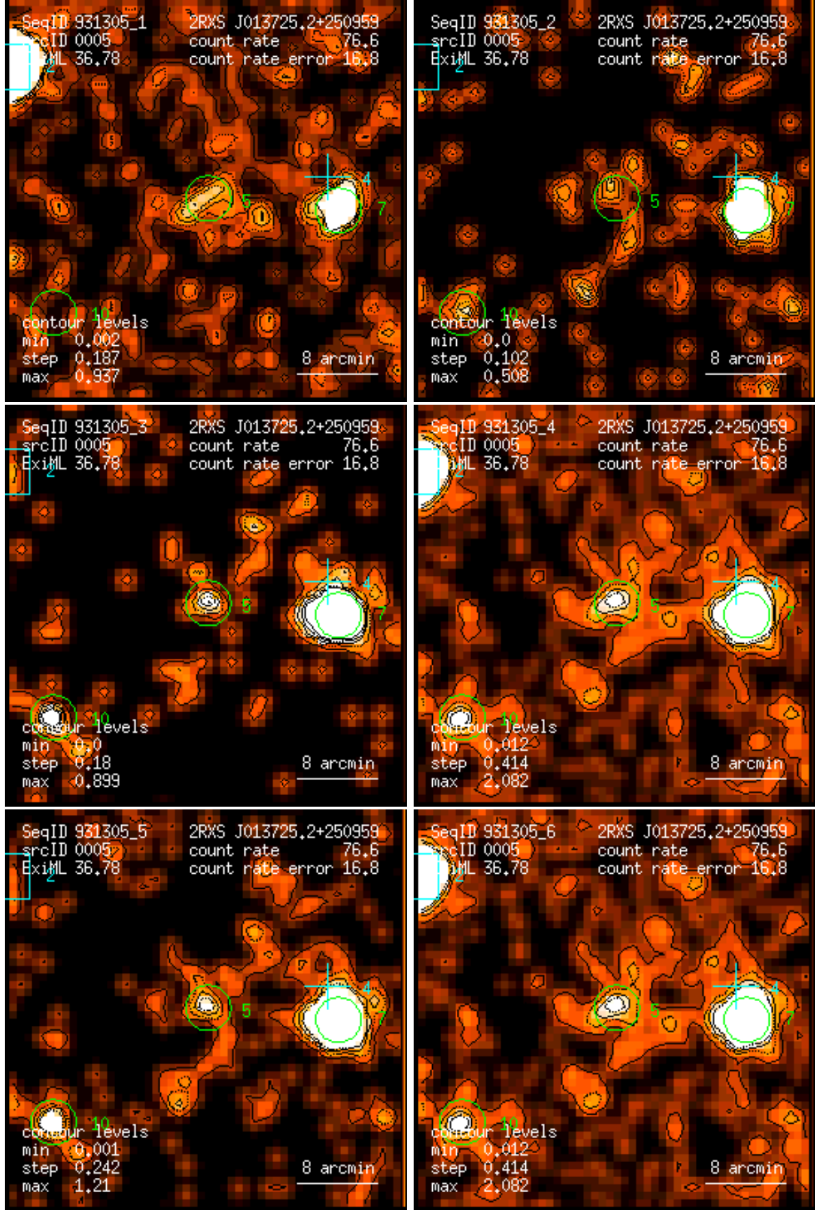
Figure 5: RASS 931305: detection 0005: band rate images, Gaussian filter: (1) PSPC channels 11 – 41, (2) 52 – 90, (3) 91 – 201, (4) 11 – 235, (5) 52 – 201, (6) 11 – 201. Broad band rates in counts/ks. Band rate contour levels in counts/ks/arcmin 2 .
