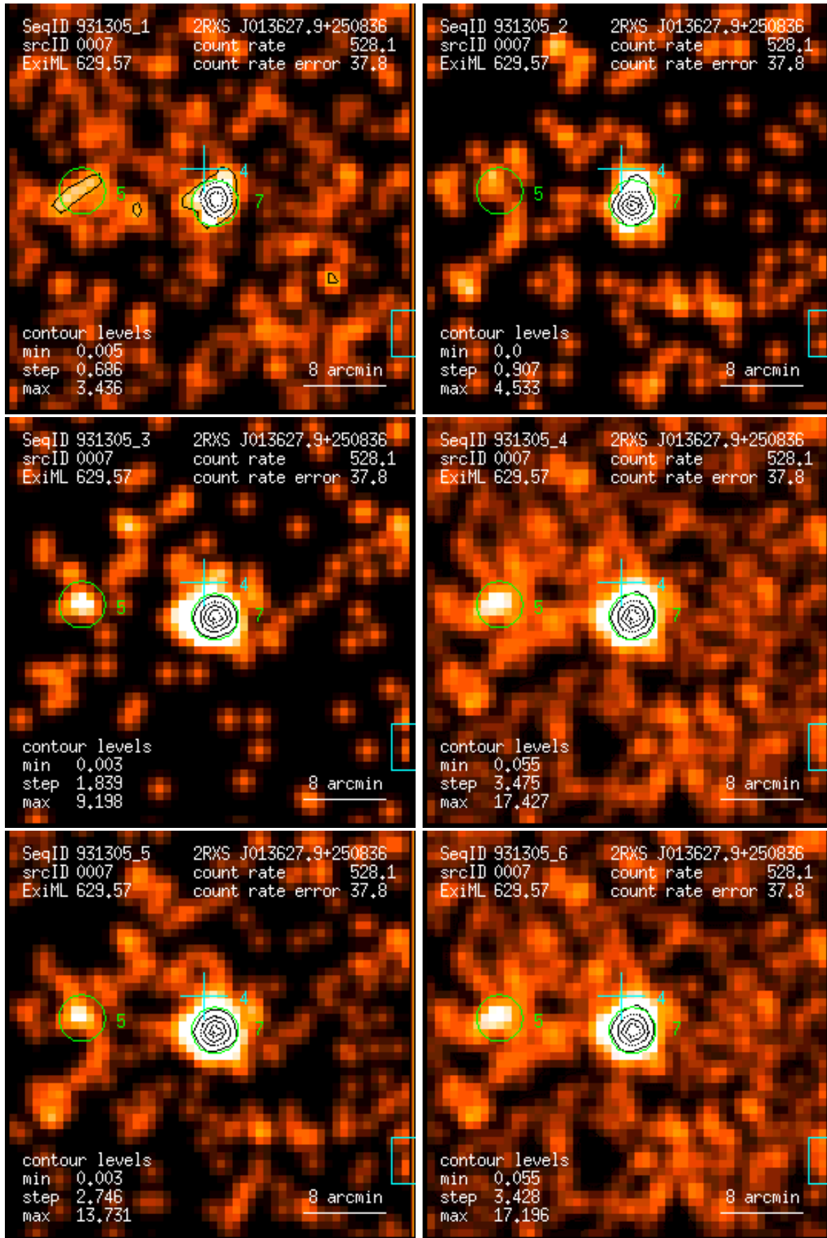
Figure 7: RASS 931305: detection 0007: band rate images, Gaussian filter: (1) PSPC channels 11 – 41, (2) 52 – 90, (3) 91 – 201, (4) 11 – 235, (5) 52 – 201, (6) 11 – 201. Broad band rates in counts/ks. Band rate contour levels in counts/ks/arcmin 2 .
