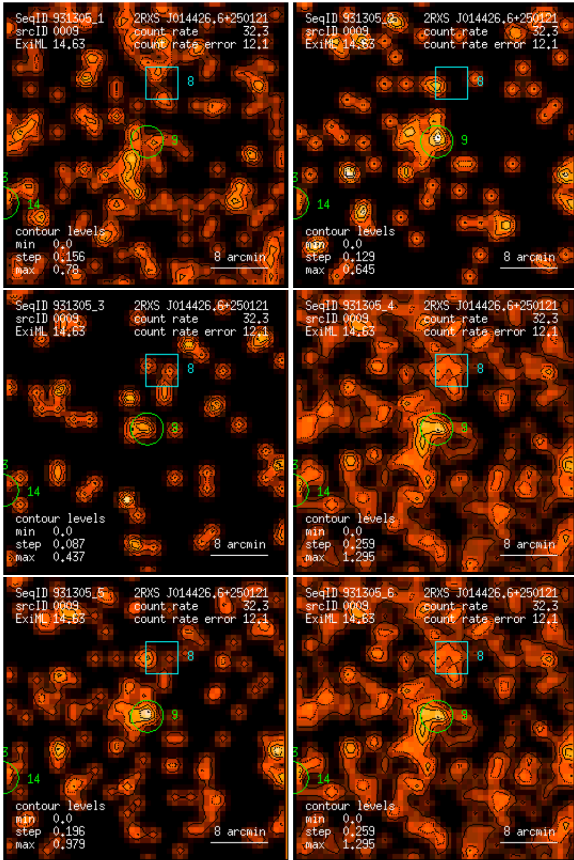
Figure 9: RASS 931305: detection 0009: band rate images, Gaussian filter: (1) PSPC channels 11 – 41, (2) 52 – 90, (3) 91 – 201, (4) 11 – 235, (5) 52 – 201, (6) 11 – 201. Broad band rates in counts/ks. Band rate contour levels in counts/ks/arcmin 2 .
