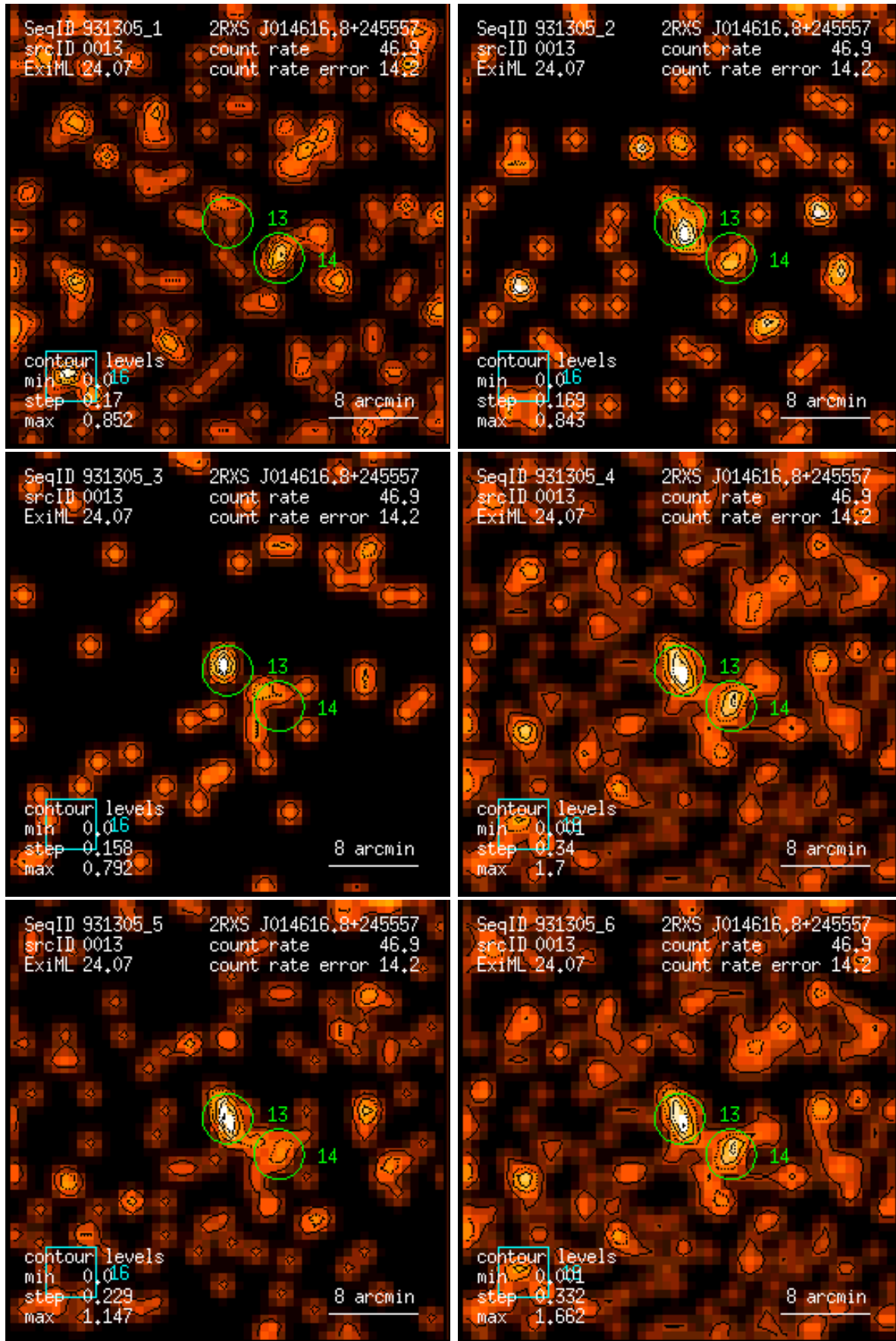
Figure 13: RASS 931305: detection 0013: band rate images, Gaussian filter: (1) PSPC channels 11 – 41, (2) 52 – 90, (3) 91 – 201, (4) 11 – 235, (5) 52 – 201, (6) 11 – 201. Broad band rates in counts/ks. Band rate contour levels in counts/ks/arcmin 2 .
