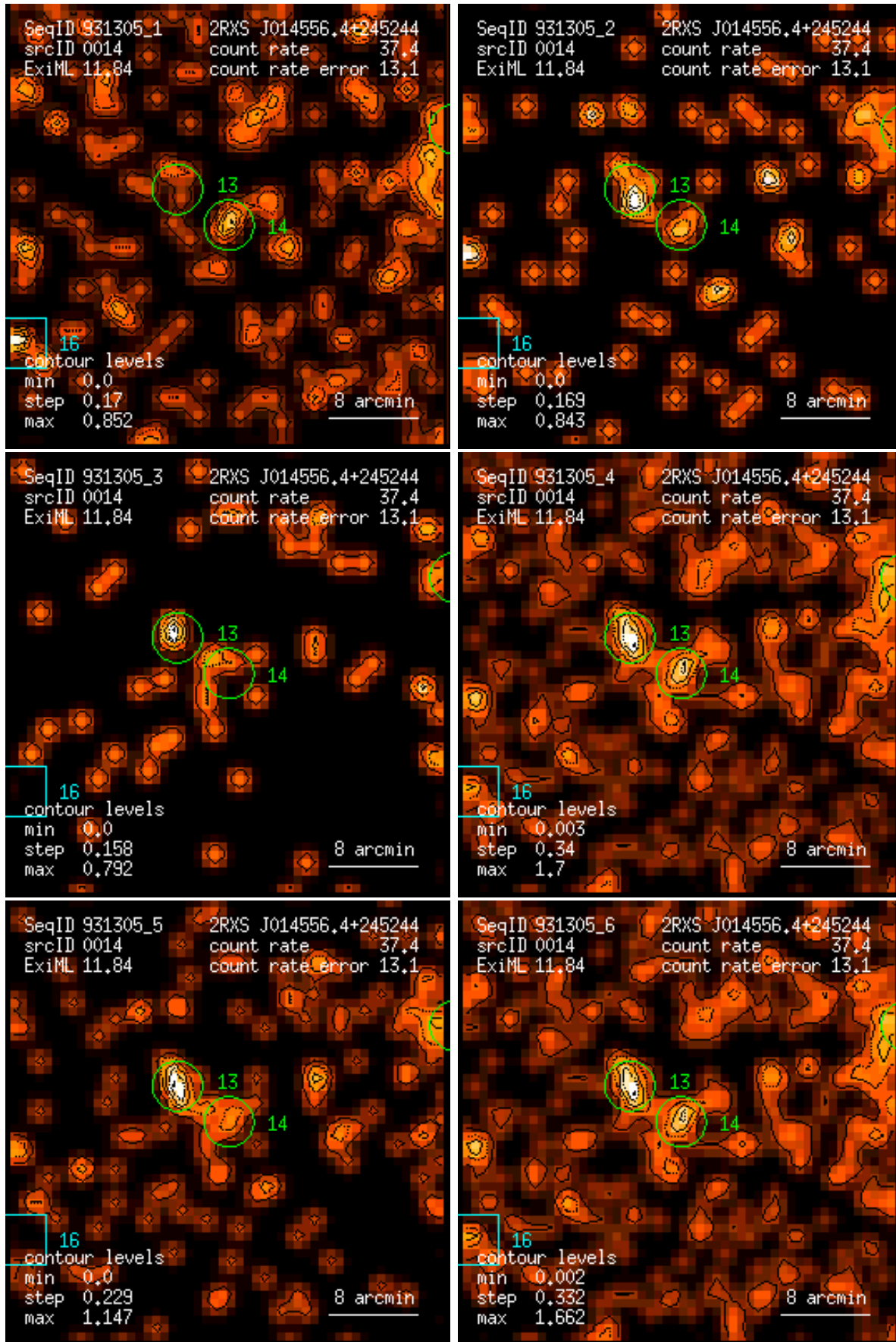
Figure 14: RASS 931305: detection 0014: band rate images, Gaussian filter: (1) PSPC channels 11 – 41, (2) 52 – 90, (3) 91 – 201, (4) 11 – 235, (5) 52 – 201, (6) 11 – 201. Broad band rates in counts/ks. Band rate contour levels in counts/ks/arcmin 2 .
