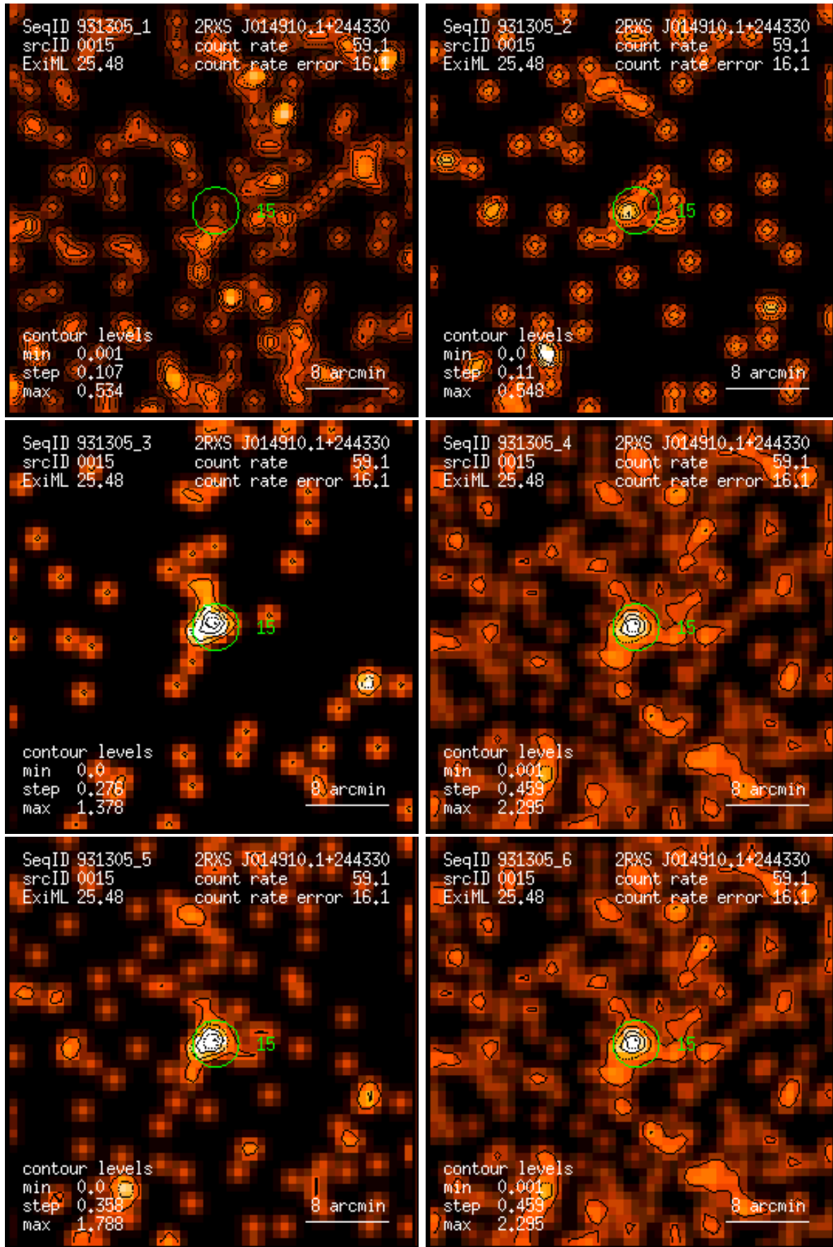
Figure 15: RASS 931305: detection 0015: band rate images, Gaussian filter: (1) PSPC channels 11 – 41, (2) 52 – 90, (3) 91 – 201, (4) 11 – 235, (5) 52 – 201, (6) 11 – 201. Broad band rates in counts/ks. Band rate contour levels in counts/ks/arcmin 2 .
