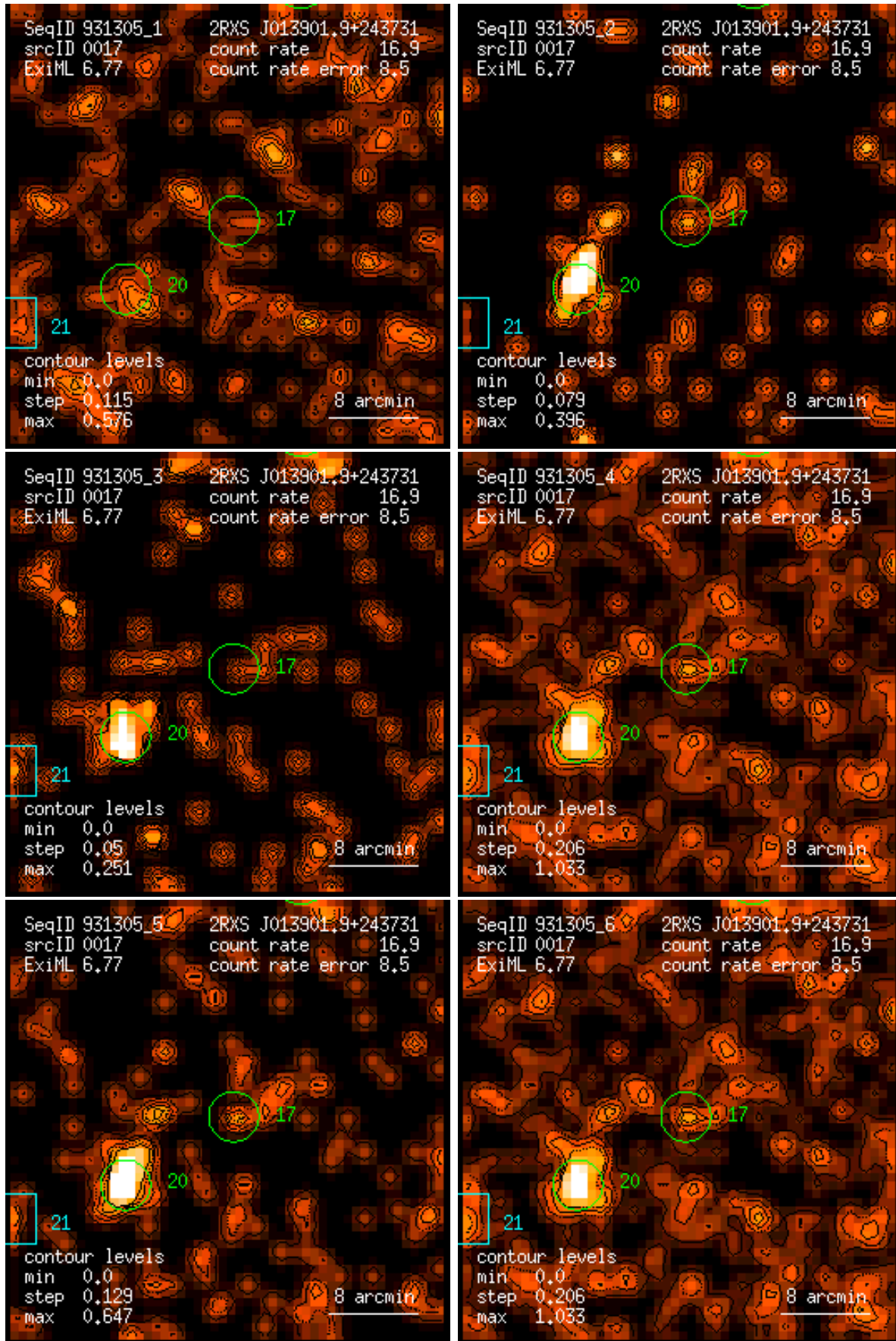
Figure 17: RASS 931305: detection 0017: band rate images, Gaussian filter: (1) PSPC channels 11 – 41, (2) 52 – 90, (3) 91 – 201, (4) 11 – 235, (5) 52 – 201, (6) 11 – 201. Broad band rates in counts/ks. Band rate contour levels in counts/ks/arcmin 2 .
