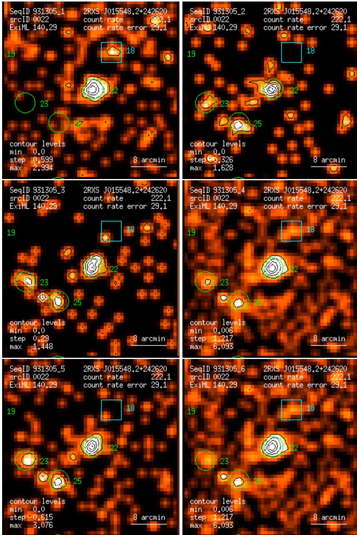
Figure 22: RASS 931305: detection 0022: band rate images, Gaussian filter: (1) PSPC channels 11 – 41, (2) 52 – 90, (3) 91 – 201, (4) 11 – 235, (5) 52 – 201, (6) 11 – 201. Broad band rates in counts/ks. Band rate contour levels in counts/ks/arcmin 2 .
