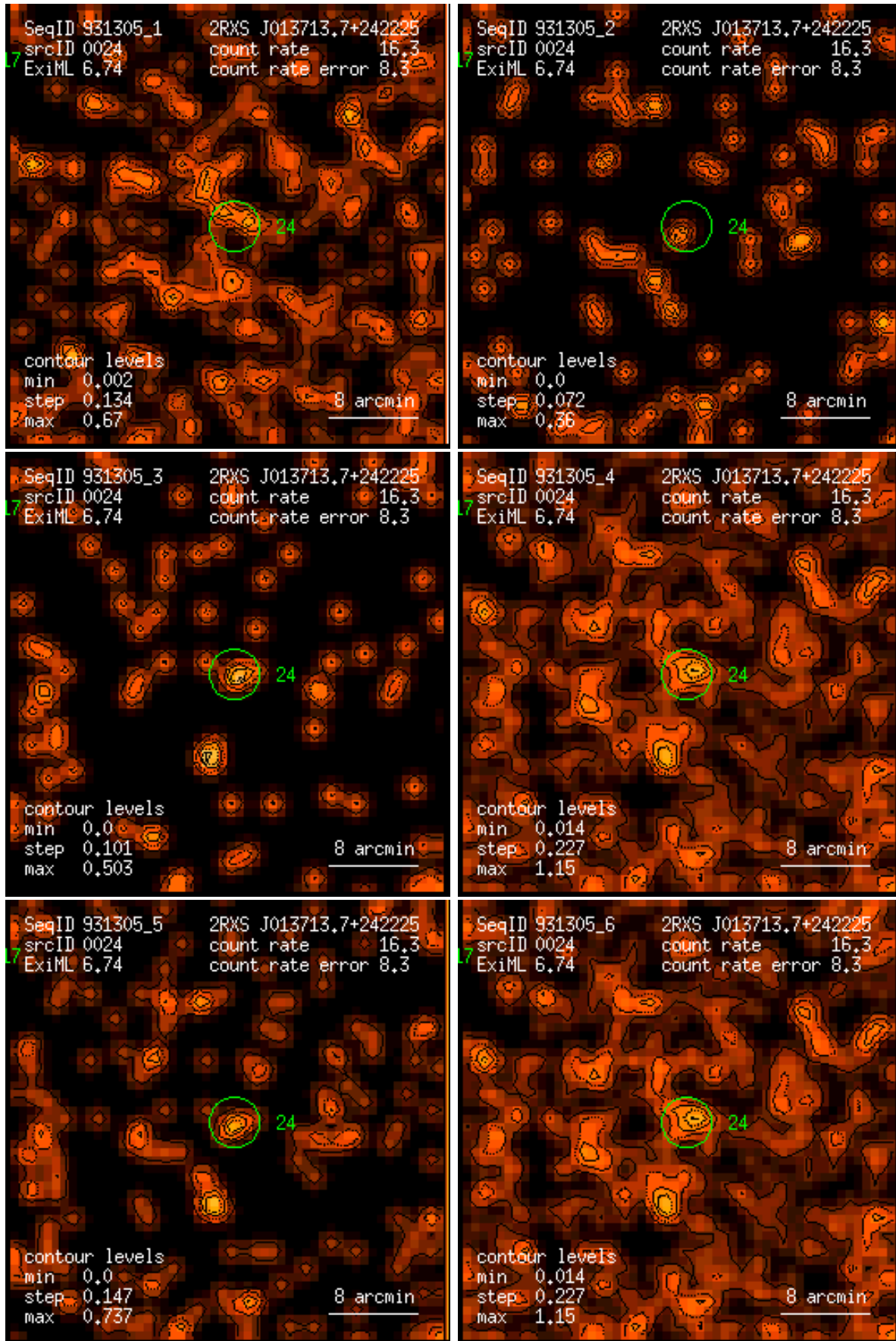
Figure 24: RASS 931305: detection 0024: band rate images, Gaussian filter: (1) PSPC channels 11 – 41, (2) 52 – 90, (3) 91 – 201, (4) 11 – 235, (5) 52 – 201, (6) 11 – 201. Broad band rates in counts/ks. Band rate contour levels in counts/ks/arcmin 2 .
