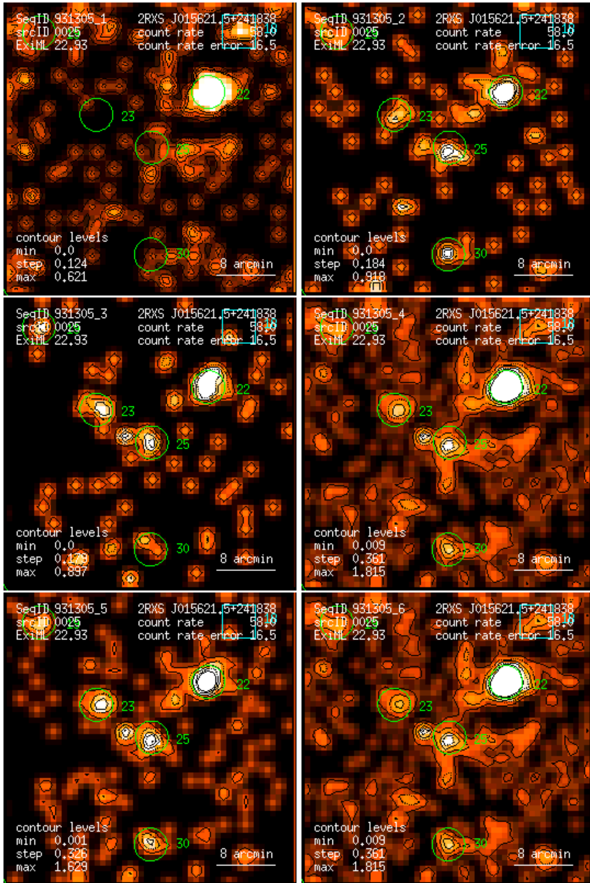
Figure 25: RASS 931305: detection 0025: band rate images, Gaussian filter: (1) PSPC channels 11 – 41, (2) 52 – 90, (3) 91 – 201, (4) 11 – 235, (5) 52 – 201, (6) 11 – 201. Broad band rates in counts/ks. Band rate contour levels in counts/ks/arcmin 2 .
