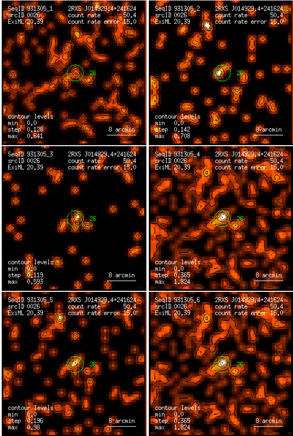
Figure 26: RASS 931305: detection 0026: band rate images, Gaussian filter: (1) PSPC channels 11 – 41, (2) 52 – 90, (3) 91 – 201, (4) 11 – 235, (5) 52 – 201, (6) 11 – 201. Broad band rates in counts/ks. Band rate contour levels in counts/ks/arcmin 2 .
