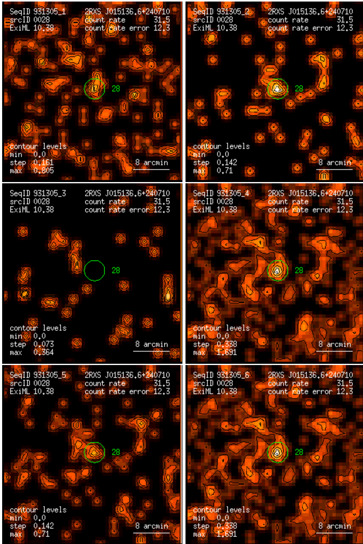
Figure 28: RASS 931305: detection 0028: band rate images, Gaussian filter: (1) PSPC channels 11 – 41, (2) 52 – 90, (3) 91 – 201, (4) 11 – 235, (5) 52 – 201, (6) 11 – 201. Broad band rates in counts/ks. Band rate contour levels in counts/ks/arcmin 2 .
