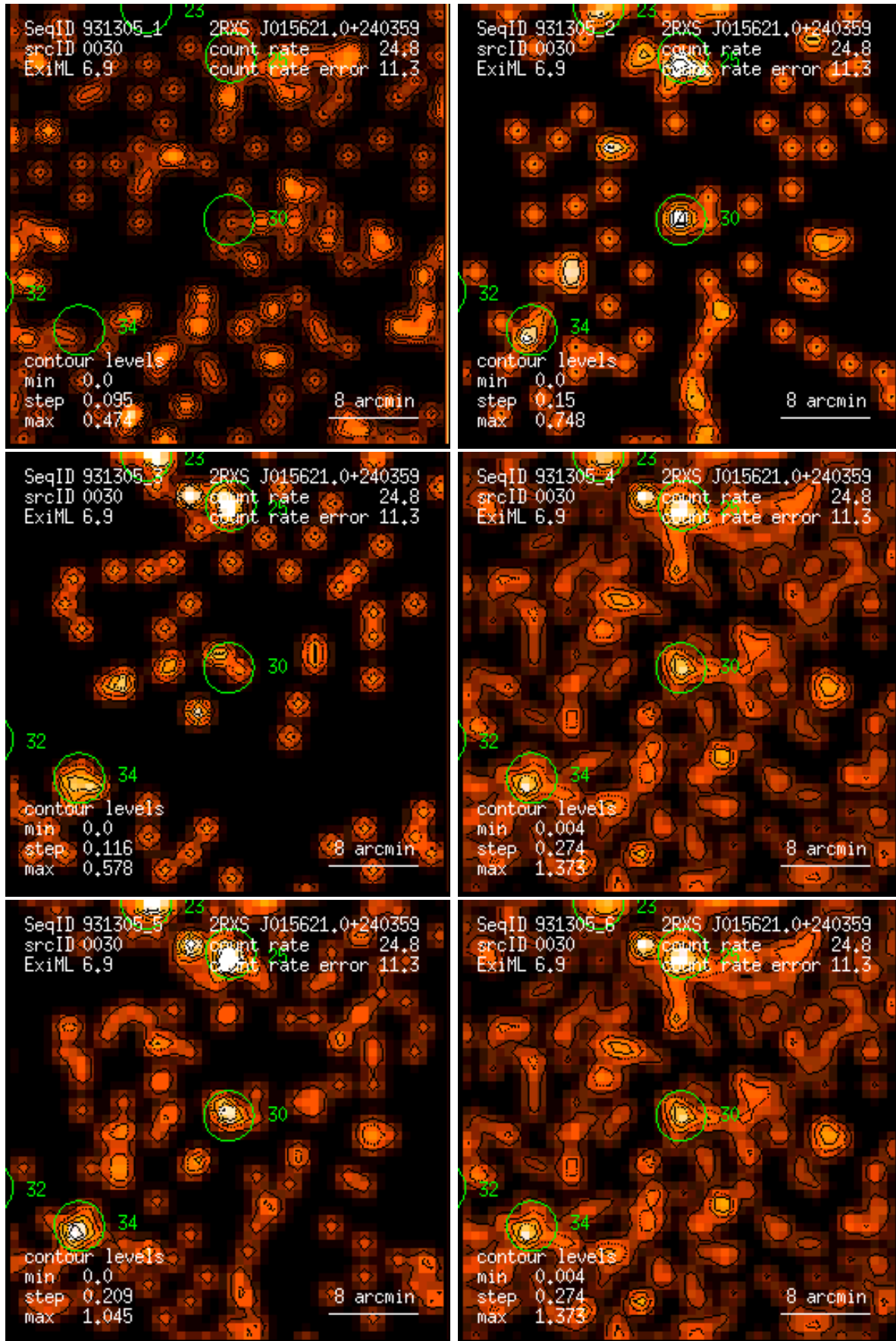
Figure 30: RASS 931305: detection 0030: band rate images, Gaussian filter: (1) PSPC channels 11 – 41, (2) 52 – 90, (3) 91 – 201, (4) 11 – 235, (5) 52 – 201, (6) 11 – 201. Broad band rates in counts/ks. Band rate contour levels in counts/ks/arcmin 2 .
