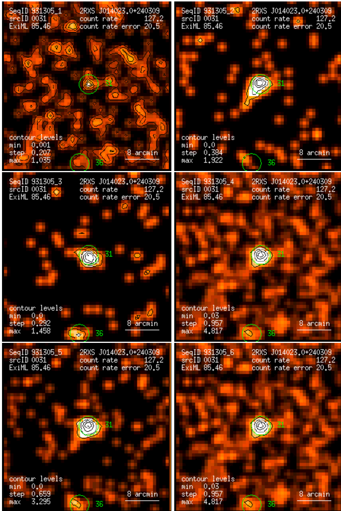
Figure 31: RASS 931305: detection 0031: band rate images, Gaussian filter: (1) PSPC channels 11 – 41, (2) 52 – 90, (3) 91 – 201, (4) 11 – 235, (5) 52 – 201, (6) 11 – 201. Broad band rates in counts/ks. Band rate contour levels in counts/ks/arcmin 2 .
