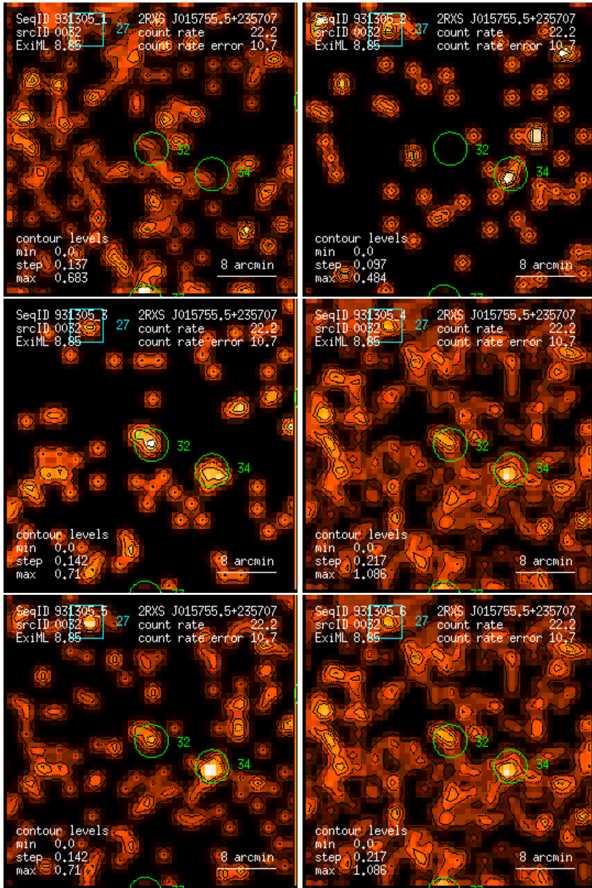
Figure 32: RASS 931305: detection 0032: band rate images, Gaussian filter: (1) PSPC channels 11 – 41, (2) 52 – 90, (3) 91 – 201, (4) 11 – 235, (5) 52 – 201, (6) 11 – 201. Broad band rates in counts/ks. Band rate contour levels in counts/ks/arcmin 2 .
