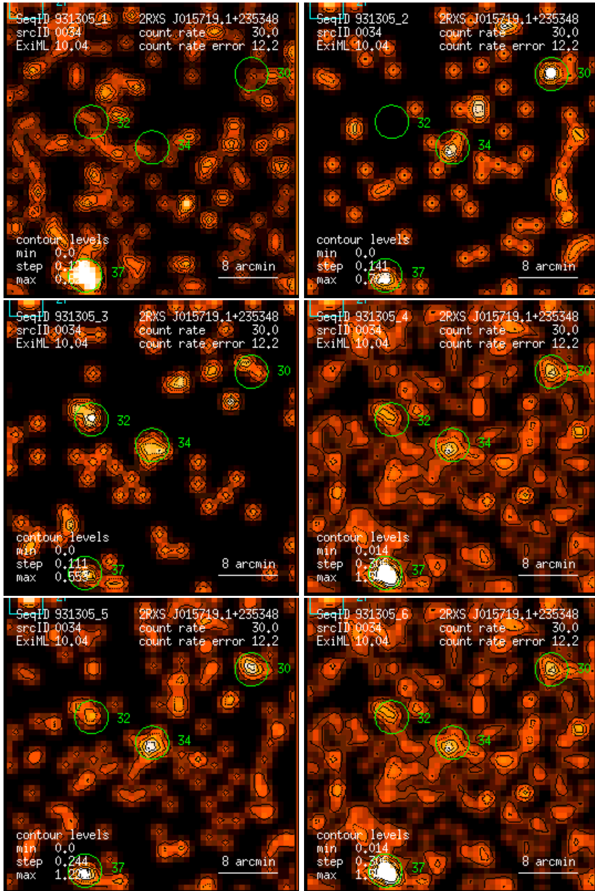
Figure 34: RASS 931305: detection 0034: band rate images, Gaussian filter: (1) PSPC channels 11 – 41, (2) 52 – 90, (3) 91 – 201, (4) 11 – 235, (5) 52 – 201, (6) 11 – 201. Broad band rates in counts/ks. Band rate contour levels in counts/ks/arcmin 2 .
