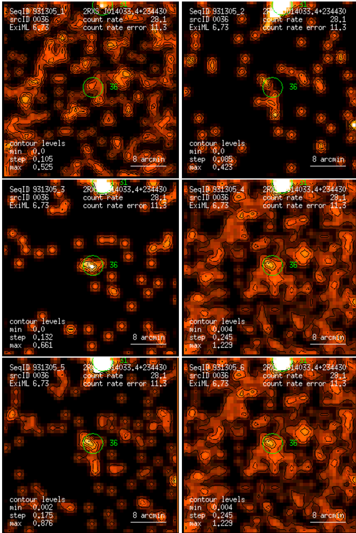
Figure 36: RASS 931305: detection 0036: band rate images, Gaussian filter: (1) PSPC channels 11 – 41, (2) 52 – 90, (3) 91 – 201, (4) 11 – 235, (5) 52 – 201, (6) 11 – 201. Broad band rates in counts/ks. Band rate contour levels in counts/ks/arcmin 2 .
