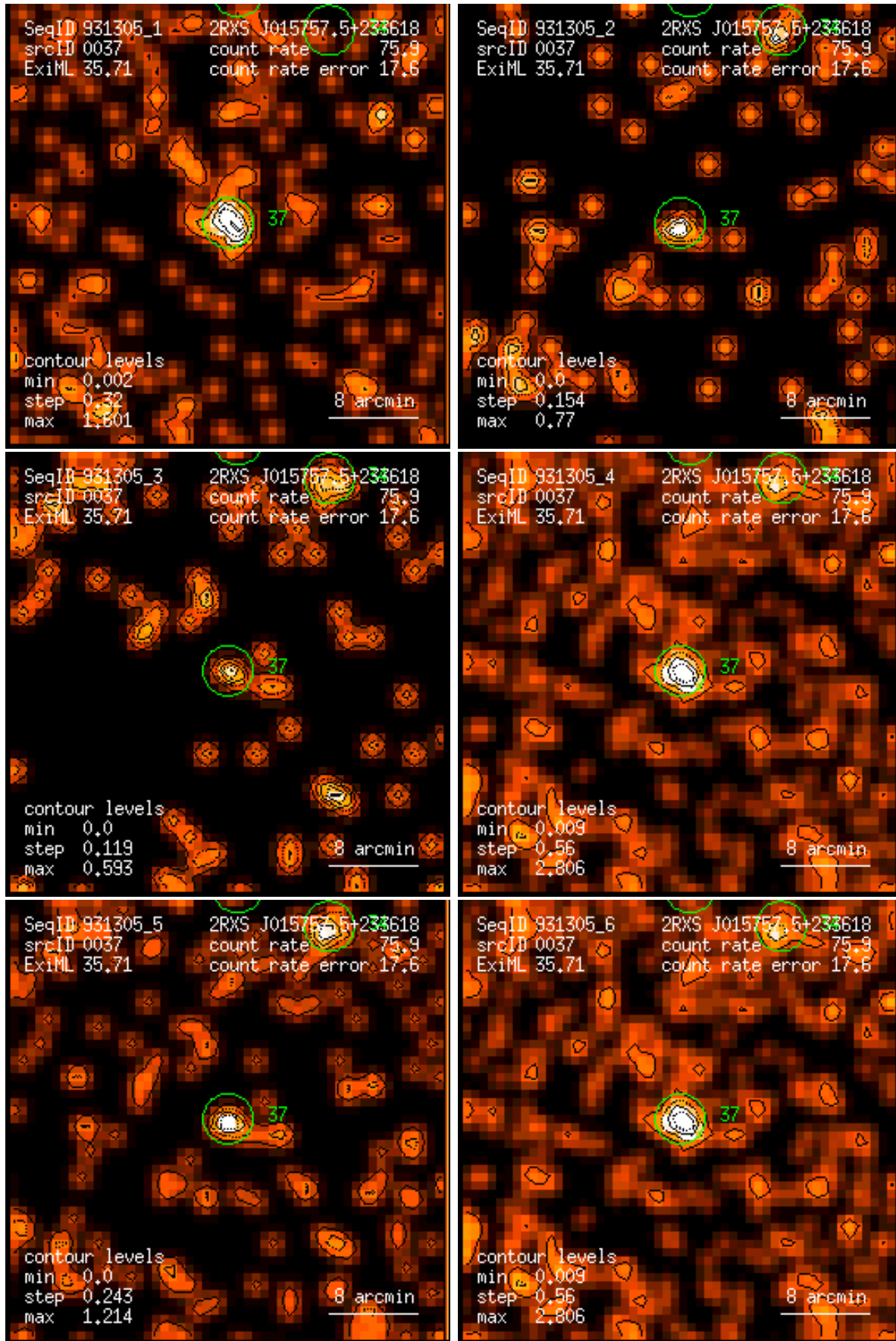
Figure 37: RASS 931305: detection 0037: band rate images, Gaussian filter: (1) PSPC channels 11 – 41, (2) 52 – 90, (3) 91 – 201, (4) 11 – 235, (5) 52 – 201, (6) 11 – 201. Broad band rates in counts/ks. Band rate contour levels in counts/ks/arcmin 2 .
