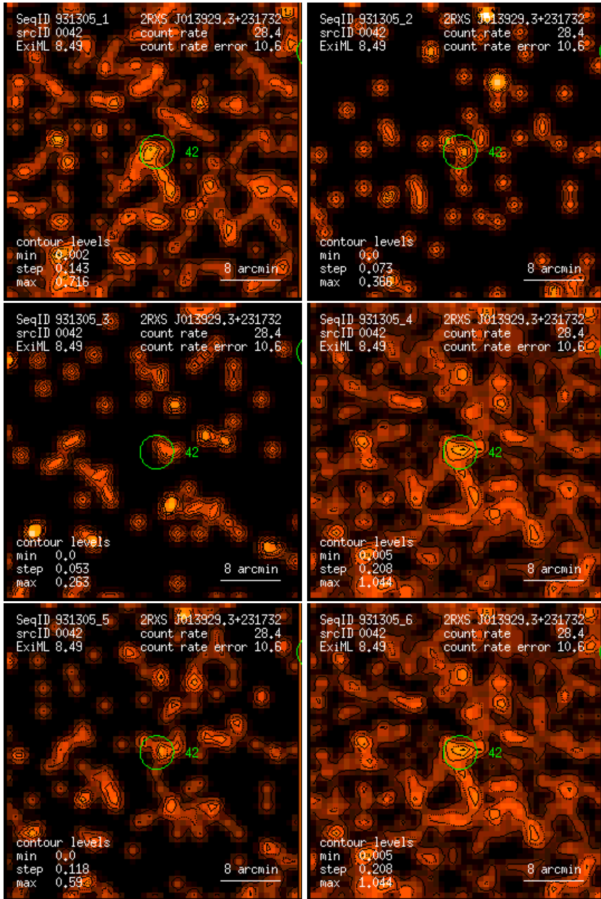
Figure 42: RASS 931305: detection 0042: band rate images, Gaussian filter: (1) PSPC channels 11 – 41, (2) 52 – 90, (3) 91 – 201, (4) 11 – 235, (5) 52 – 201, (6) 11 – 201. Broad band rates in counts/ks. Band rate contour levels in counts/ks/arcmin 2 .
