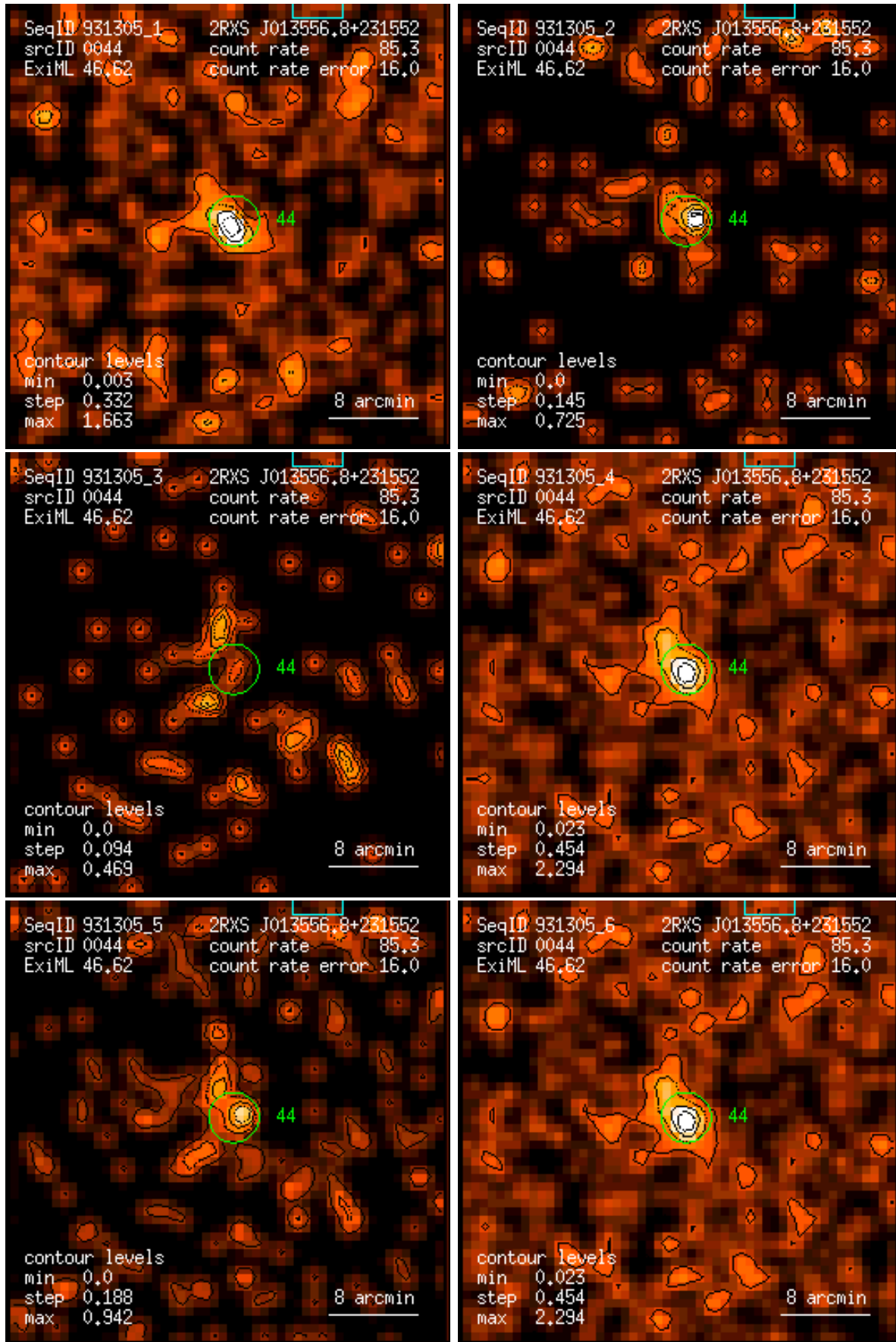
Figure 44: RASS 931305: detection 0044: band rate images, Gaussian filter: (1) PSPC channels 11 – 41, (2) 52 – 90, (3) 91 – 201, (4) 11 – 235, (5) 52 – 201, (6) 11 – 201. Broad band rates in counts/ks. Band rate contour levels in counts/ks/arcmin 2 .
