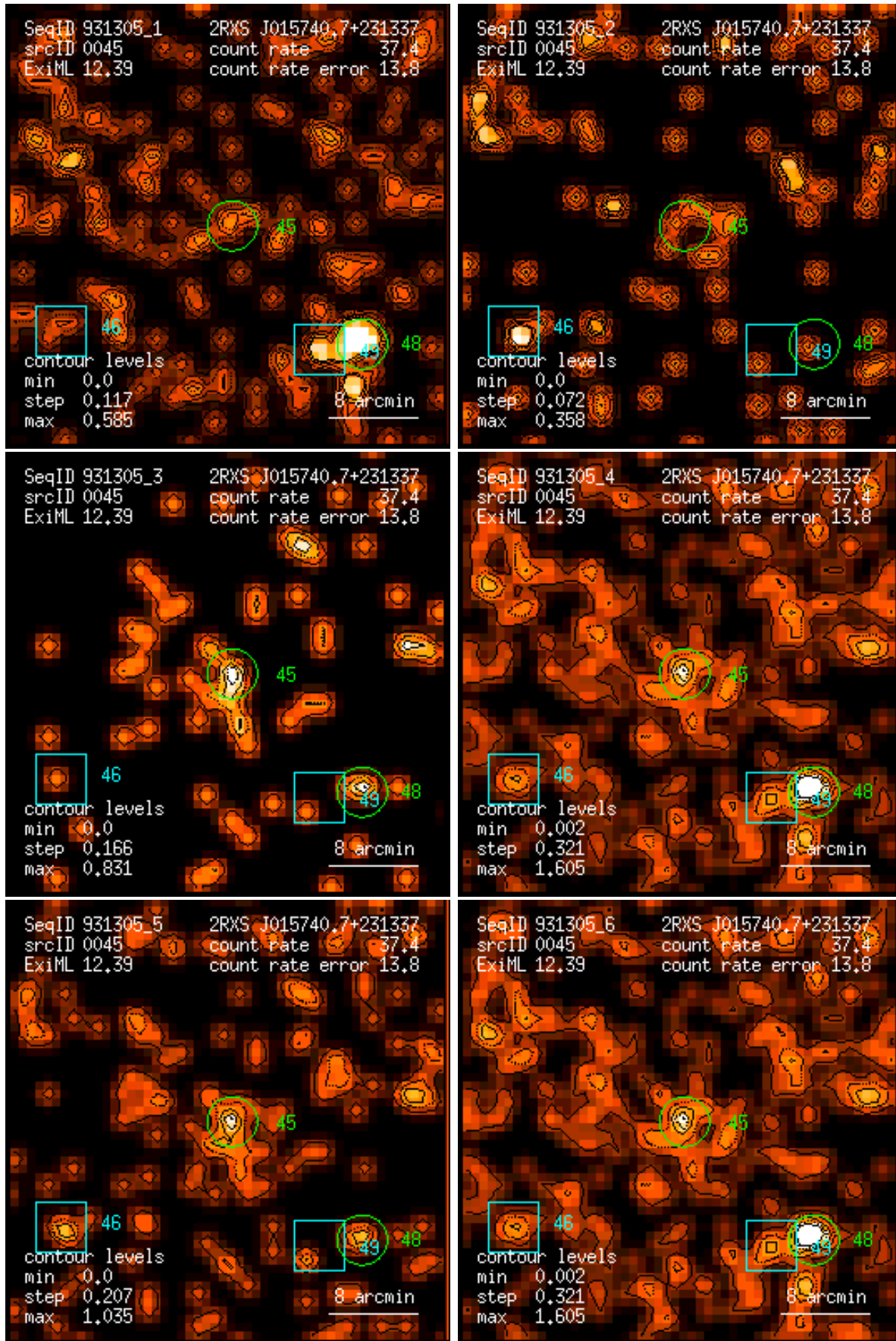
Figure 45: RASS 931305: detection 0045: band rate images, Gaussian filter: (1) PSPC channels 11 – 41, (2) 52 – 90, (3) 91 – 201, (4) 11 – 235, (5) 52 – 201, (6) 11 – 201. Broad band rates in counts/ks. Band rate contour levels in counts/ks/arcmin 2 .
