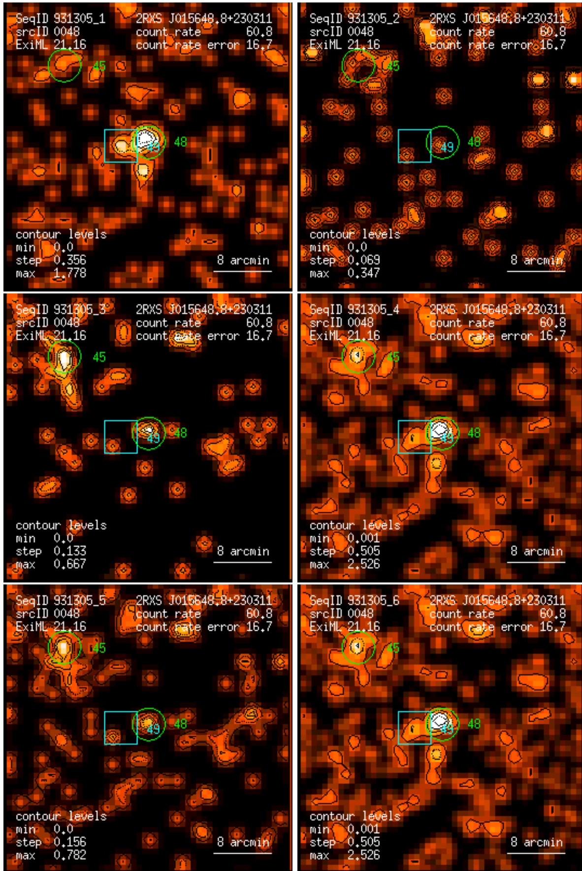
Figure 48: RASS 931305: detection 0048: band rate images, Gaussian filter: (1) PSPC channels 11 – 41, (2) 52 – 90, (3) 91 – 201, (4) 11 – 235, (5) 52 – 201, (6) 11 – 201. Broad band rates in counts/ks. Band rate contour levels in counts/ks/arcmin 2 .
