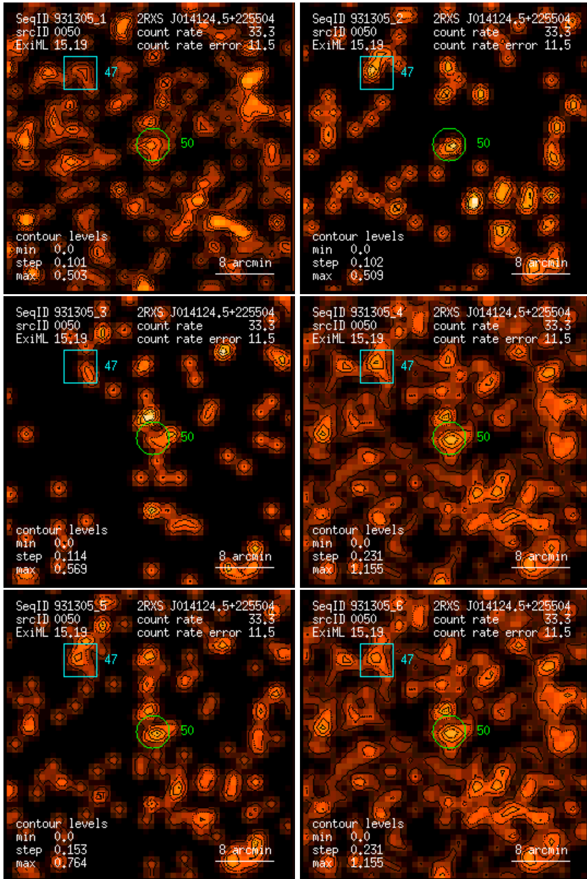
Figure 50: RASS 931305: detection 0050: band rate images, Gaussian filter: (1) PSPC channels 11 – 41, (2) 52 – 90, (3) 91 – 201, (4) 11 – 235, (5) 52 – 201, (6) 11 – 201. Broad band rates in counts/ks. Band rate contour levels in counts/ks/arcmin 2 .
