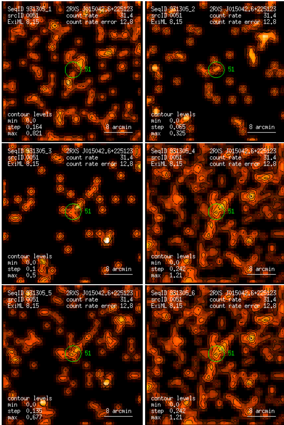
Figure 51: RASS 931305: detection 0051: band rate images, Gaussian filter: (1) PSPC channels 11 – 41, (2) 52 – 90, (3) 91 – 201, (4) 11 – 235, (5) 52 – 201, (6) 11 – 201. Broad band rates in counts/ks. Band rate contour levels in counts/ks/arcmin 2 .
