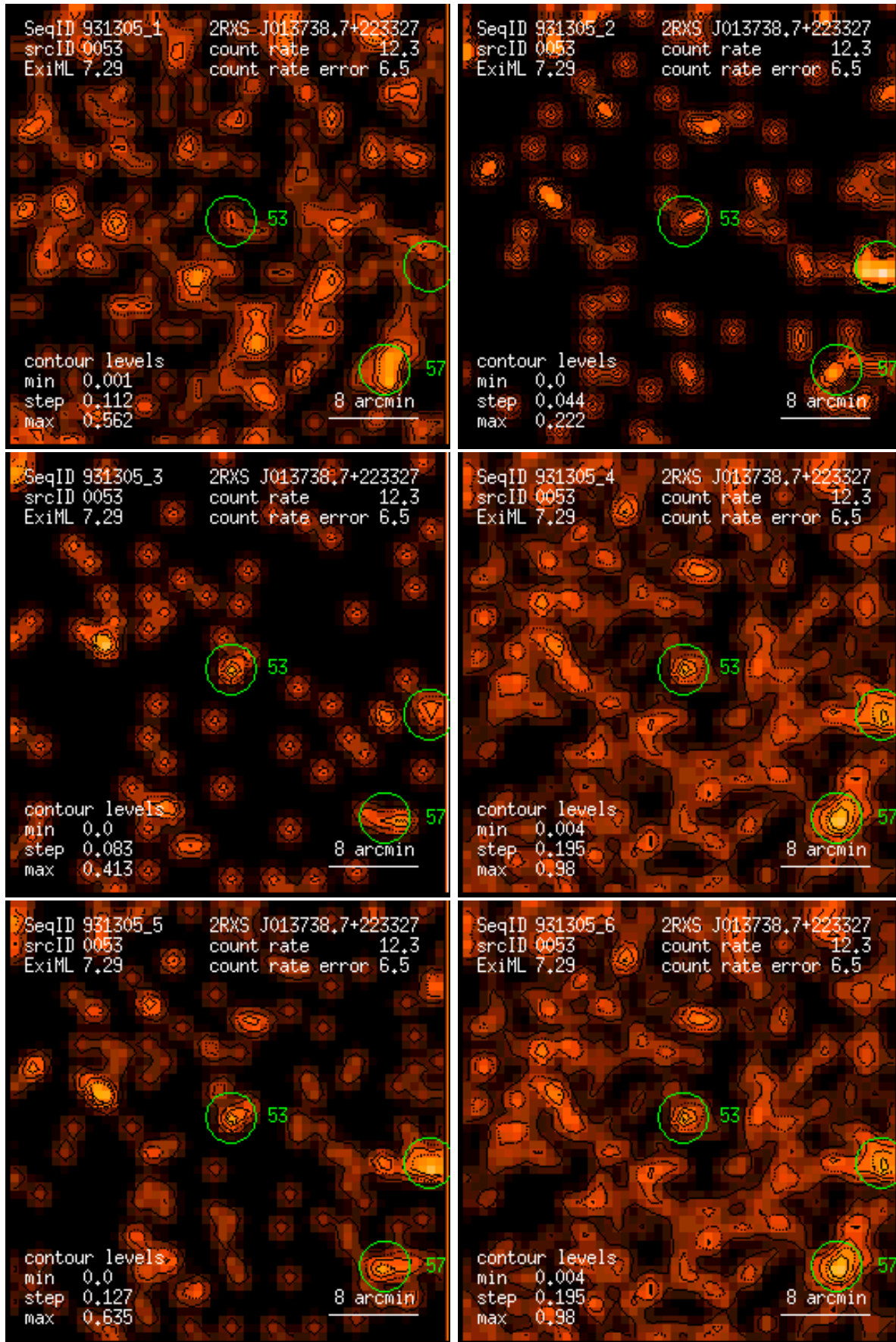
Figure 53: RASS 931305: detection 0053: band rate images, Gaussian filter: (1) PSPC channels 11 – 41, (2) 52 – 90, (3) 91 – 201, (4) 11 – 235, (5) 52 – 201, (6) 11 – 201. Broad band rates in counts/ks. Band rate contour levels in counts/ks/arcmin 2 .
