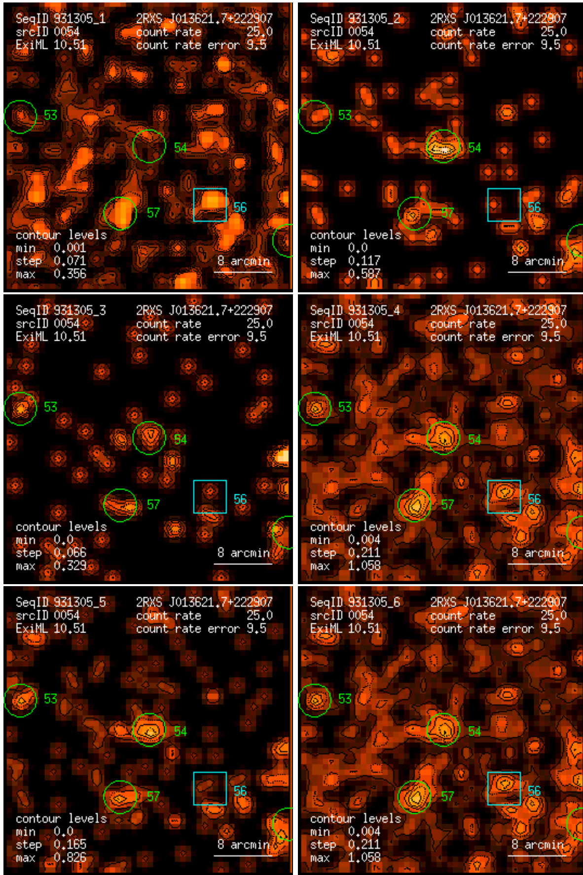
Figure 54: RASS 931305: detection 0054: band rate images, Gaussian filter: (1) PSPC channels 11 – 41, (2) 52 – 90, (3) 91 – 201, (4) 11 – 235, (5) 52 – 201, (6) 11 – 201. Broad band rates in counts/ks. Band rate contour levels in counts/ks/arcmin 2 .
