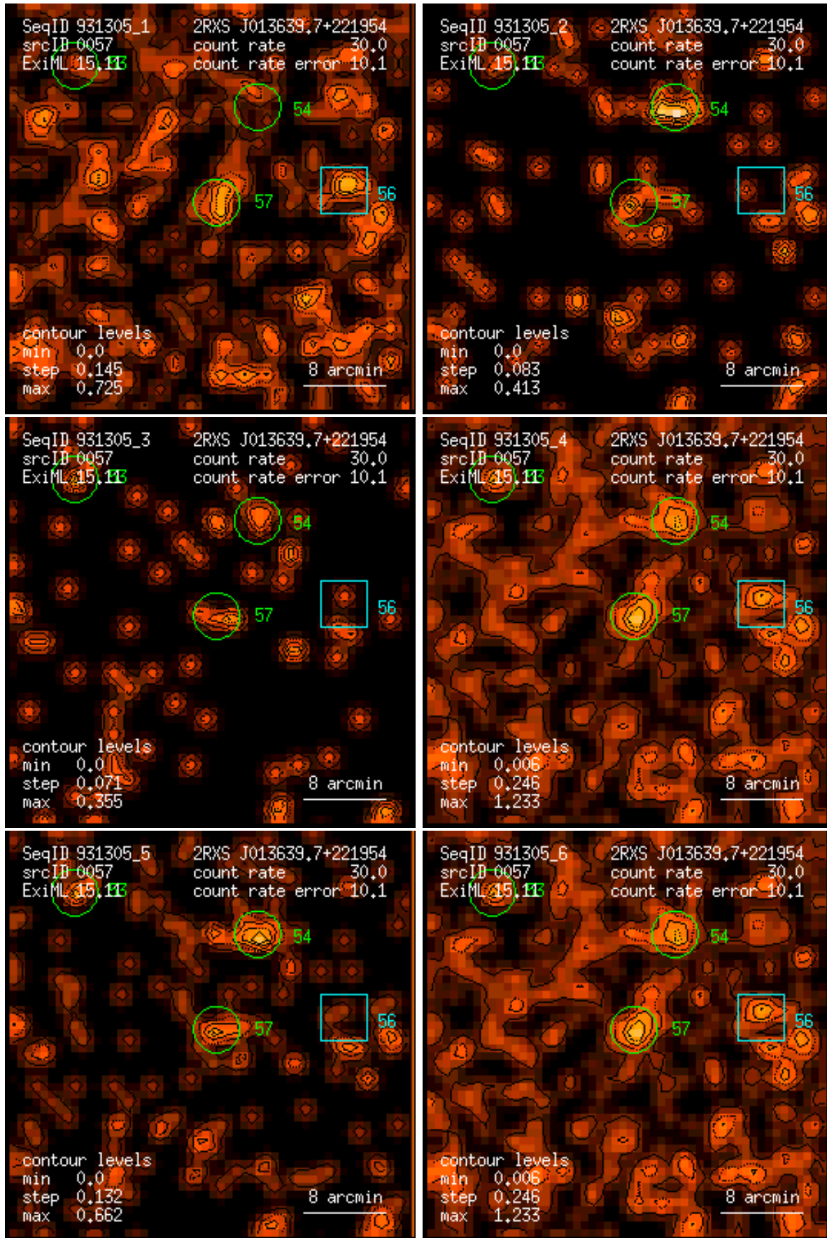
Figure 57: RASS 931305: detection 0057: band rate images, Gaussian filter: (1) PSPC channels 11 – 41, (2) 52 – 90, (3) 91 – 201, (4) 11 – 235, (5) 52 – 201, (6) 11 – 201. Broad band rates in counts/ks. Band rate contour levels in counts/ks/arcmin 2 .
