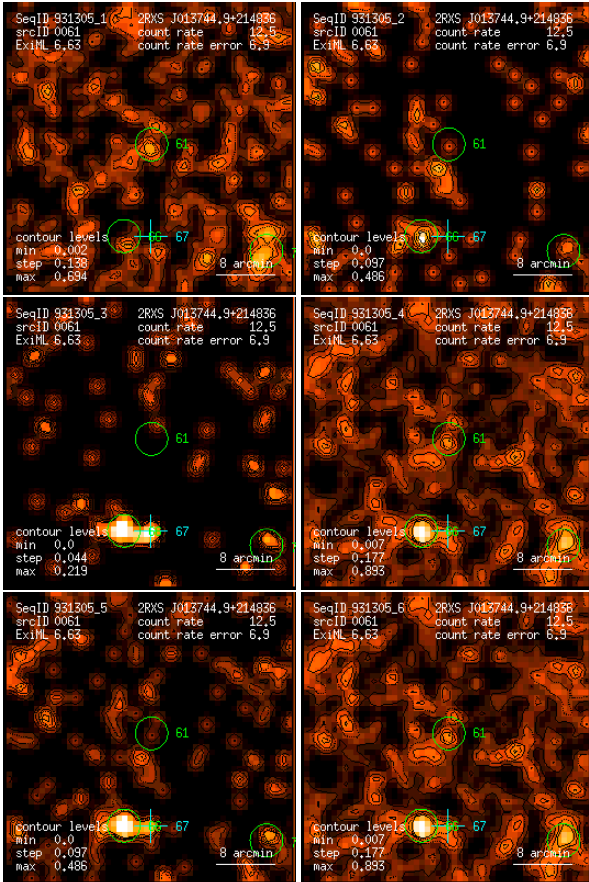
Figure 61: RASS 931305: detection 0061: band rate images, Gaussian filter: (1) PSPC channels 11 – 41, (2) 52 – 90, (3) 91 – 201, (4) 11 – 235, (5) 52 – 201, (6) 11 – 201. Broad band rates in counts/ks. Band rate contour levels in counts/ks/arcmin 2 .
