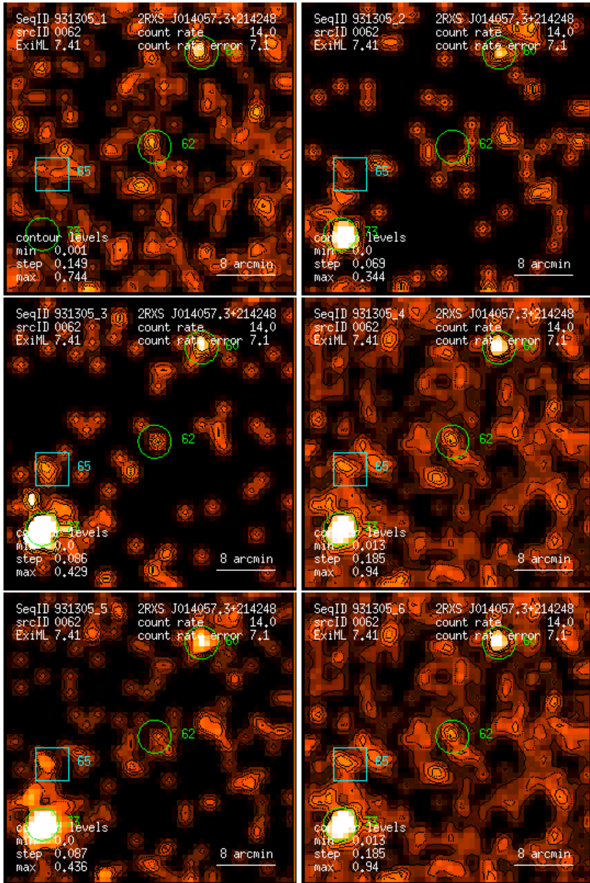
Figure 62: RASS 931305: detection 0062: band rate images, Gaussian filter: (1) PSPC channels 11 – 41, (2) 52 – 90, (3) 91 – 201, (4) 11 – 235, (5) 52 – 201, (6) 11 – 201. Broad band rates in counts/ks. Band rate contour levels in counts/ks/arcmin 2 .
