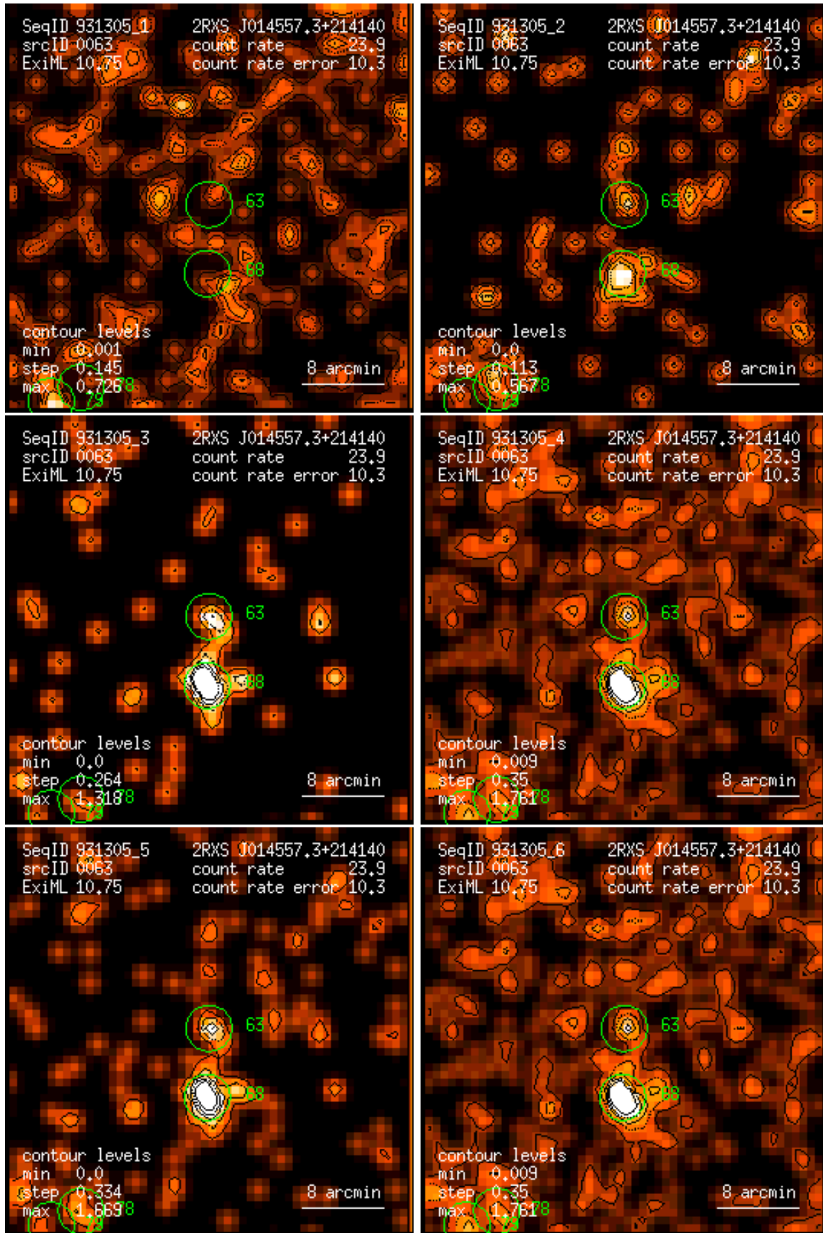
Figure 63: RASS 931305: detection 0063: band rate images, Gaussian filter: (1) PSPC channels 11 – 41, (2) 52 – 90, (3) 91 – 201, (4) 11 – 235, (5) 52 – 201, (6) 11 – 201. Broad band rates in counts/ks. Band rate contour levels in counts/ks/arcmin 2 .
