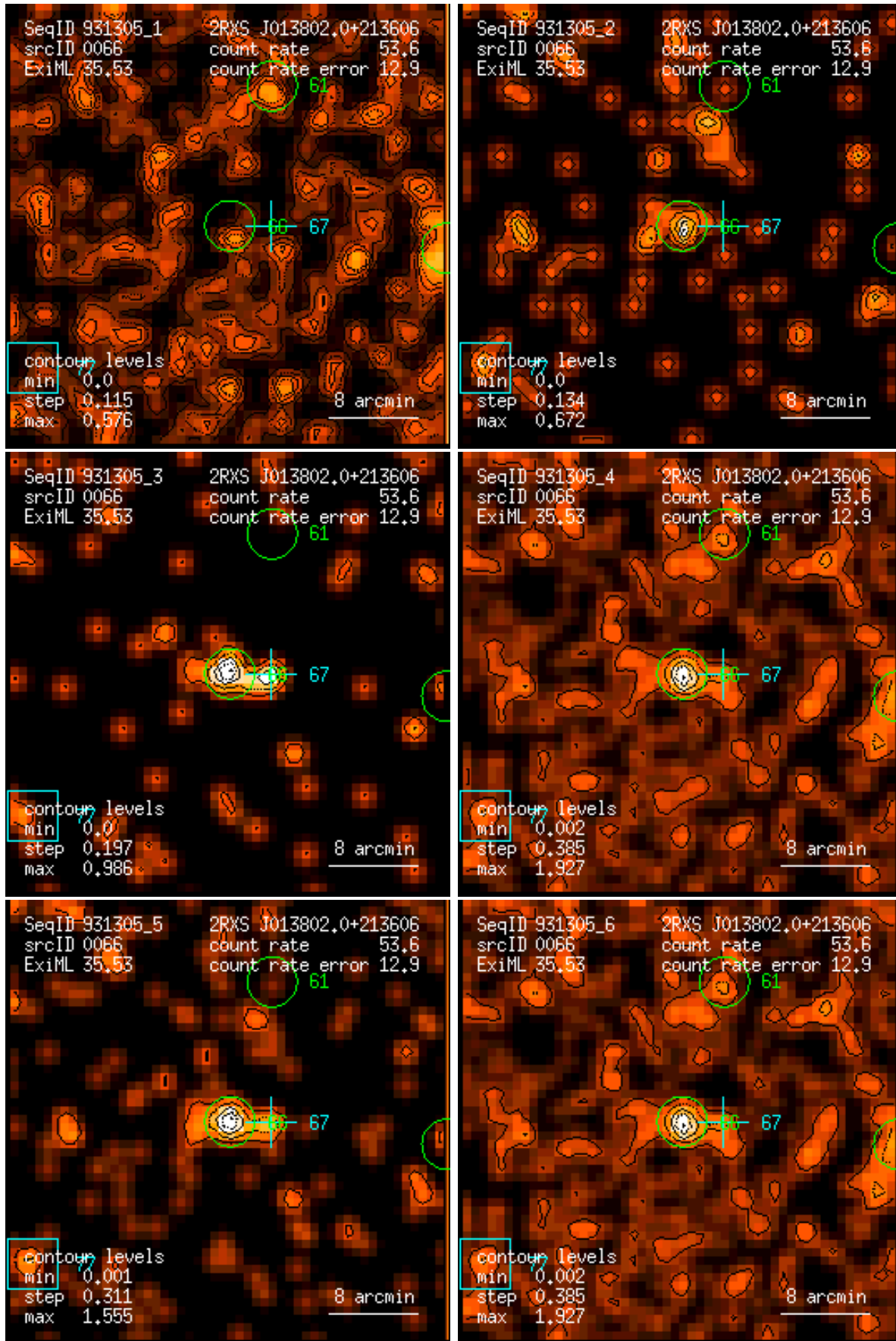
Figure 66: RASS 931305: detection 0066: band rate images, Gaussian filter: (1) PSPC channels 11 – 41, (2) 52 – 90, (3) 91 – 201, (4) 11 – 235, (5) 52 – 201, (6) 11 – 201. Broad band rates in counts/ks. Band rate contour levels in counts/ks/arcmin 2 .
