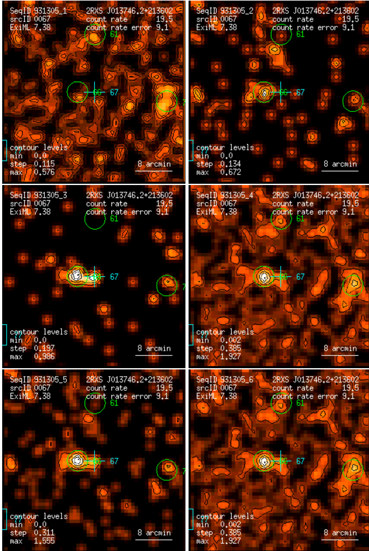
Figure 67: RASS 931305: detection 0067: band rate images, Gaussian filter: (1) PSPC channels 11 – 41, (2) 52 – 90, (3) 91 – 201, (4) 11 – 235, (5) 52 – 201, (6) 11 – 201. Broad band rates in counts/ks. Band rate contour levels in counts/ks/arcmin 2 .
