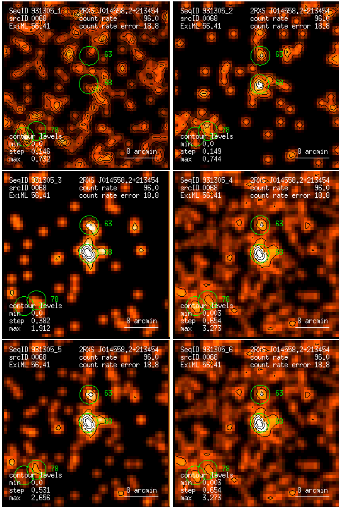
Figure 68: RASS 931305: detection 0068: band rate images, Gaussian filter: (1) PSPC channels 11 – 41, (2) 52 – 90, (3) 91 – 201, (4) 11 – 235, (5) 52 – 201, (6) 11 – 201. Broad band rates in counts/ks. Band rate contour levels in counts/ks/arcmin 2 .
