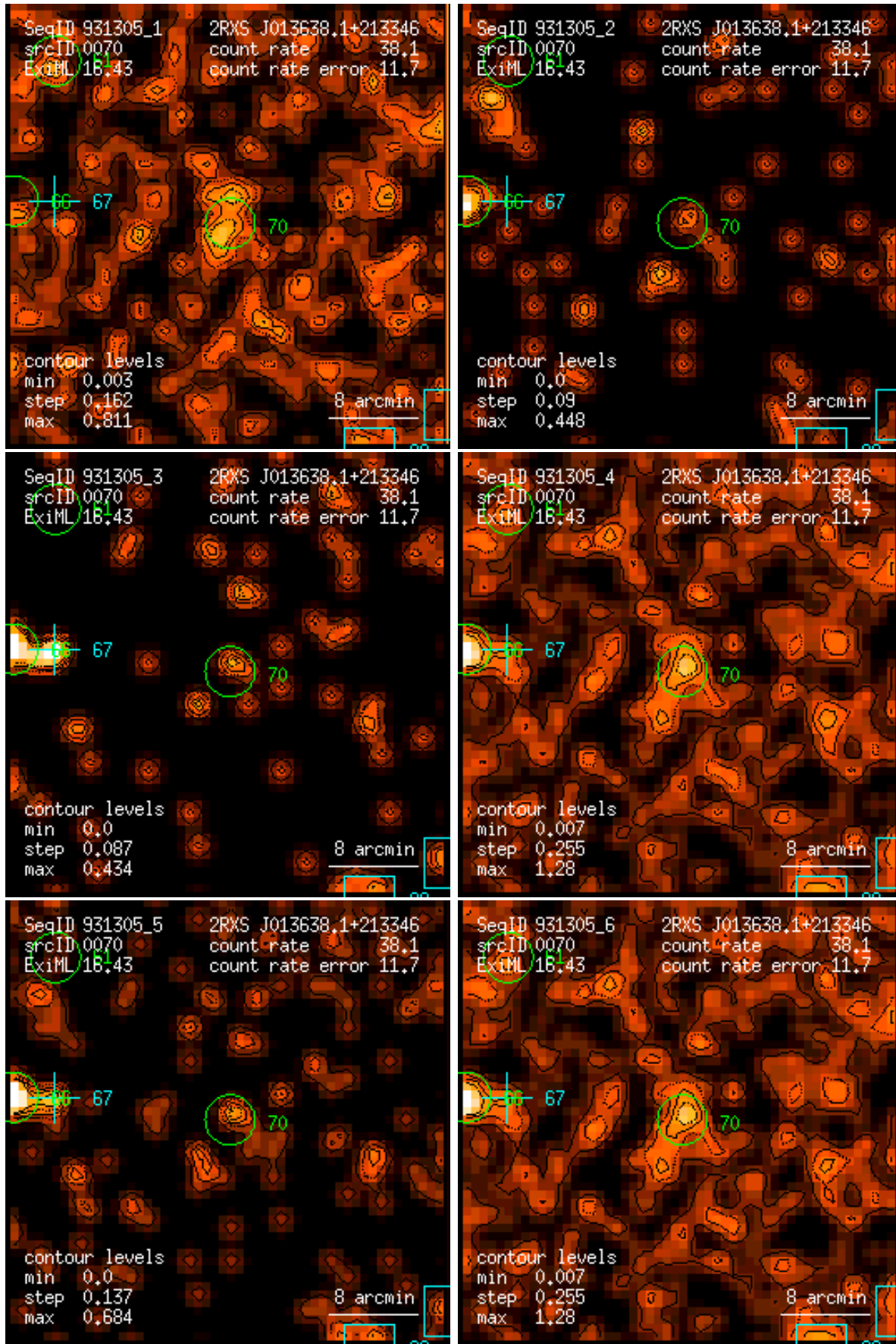
Figure 70: RASS 931305: detection 0070: band rate images, Gaussian filter: (1) PSPC channels 11 – 41, (2) 52 – 90, (3) 91 – 201, (4) 11 – 235, (5) 52 – 201, (6) 11 – 201. Broad band rates in counts/ks. Band rate contour levels in counts/ks/arcmin 2 .
