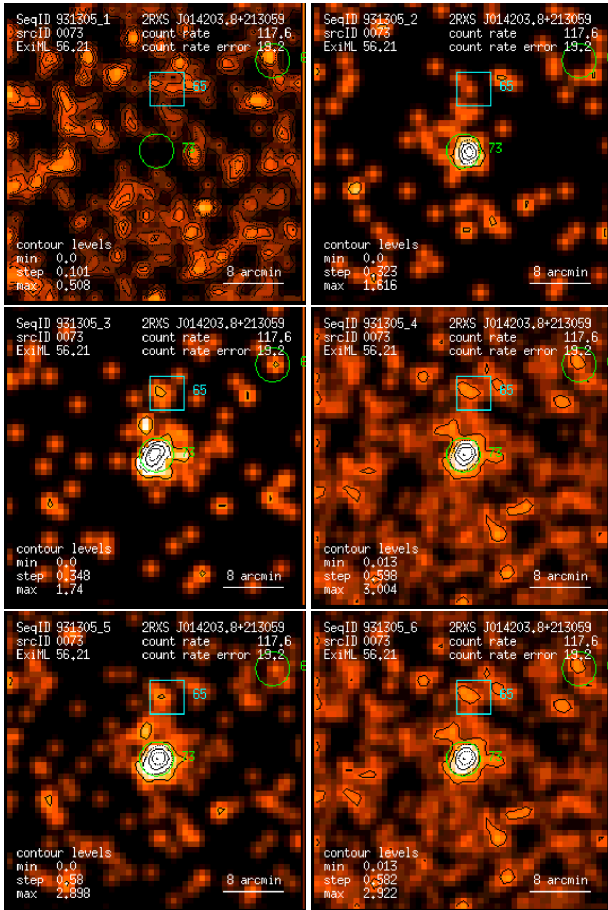
Figure 73: RASS 931305: detection 0073: band rate images, Gaussian filter: (1) PSPC channels 11 – 41, (2) 52 – 90, (3) 91 – 201, (4) 11 – 235, (5) 52 – 201, (6) 11 – 201. Broad band rates in counts/ks. Band rate contour levels in counts/ks/arcmin 2 .
