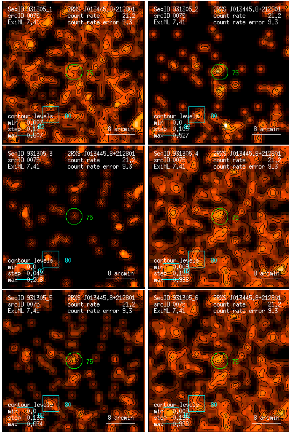
Figure 75: RASS 931305: detection 0075: band rate images, Gaussian filter: (1) PSPC channels 11 – 41, (2) 52 – 90, (3) 91 – 201, (4) 11 – 235, (5) 52 – 201, (6) 11 – 201. Broad band rates in counts/ks. Band rate contour levels in counts/ks/arcmin 2 .
