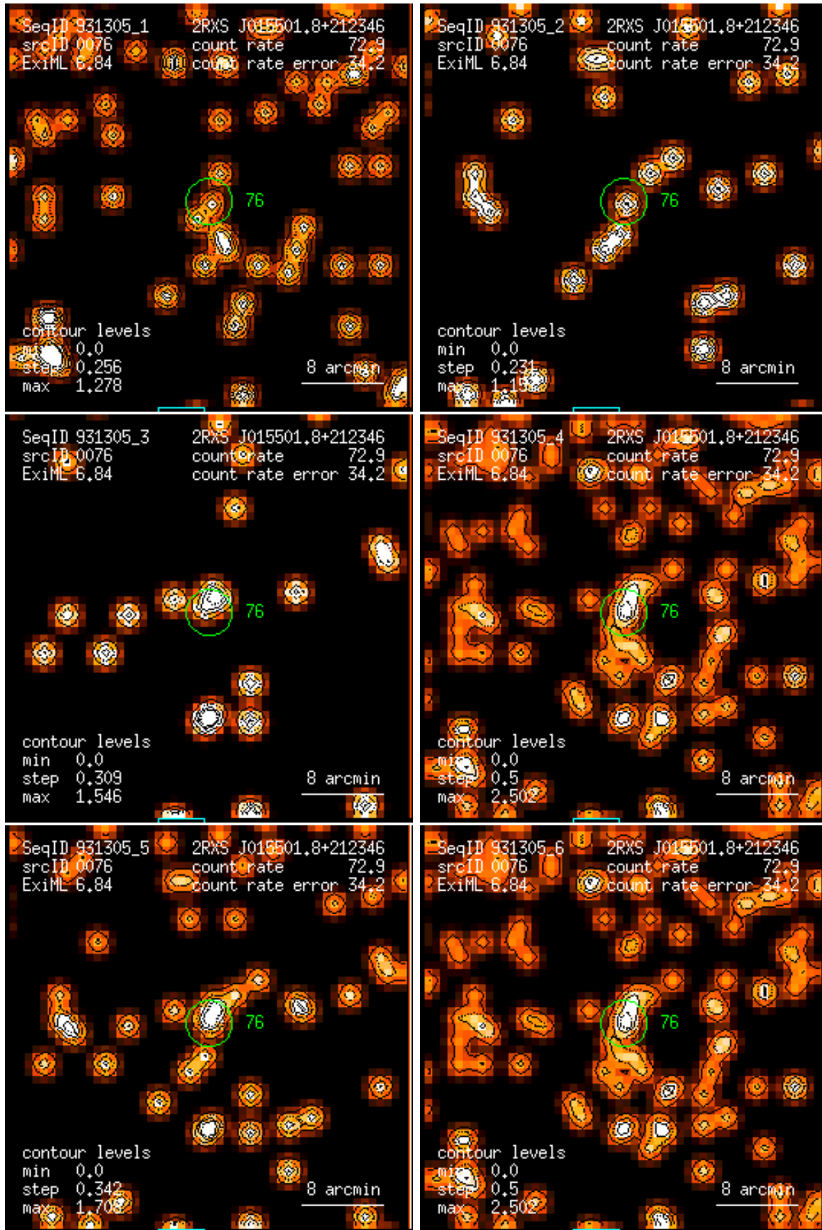
Figure 76: RASS 931305: detection 0076: band rate images, Gaussian filter: (1) PSPC channels 11 – 41, (2) 52 – 90, (3) 91 – 201, (4) 11 – 235, (5) 52 – 201, (6) 11 – 201. Broad band rates in counts/ks. Band rate contour levels in counts/ks/arcmin 2 .
