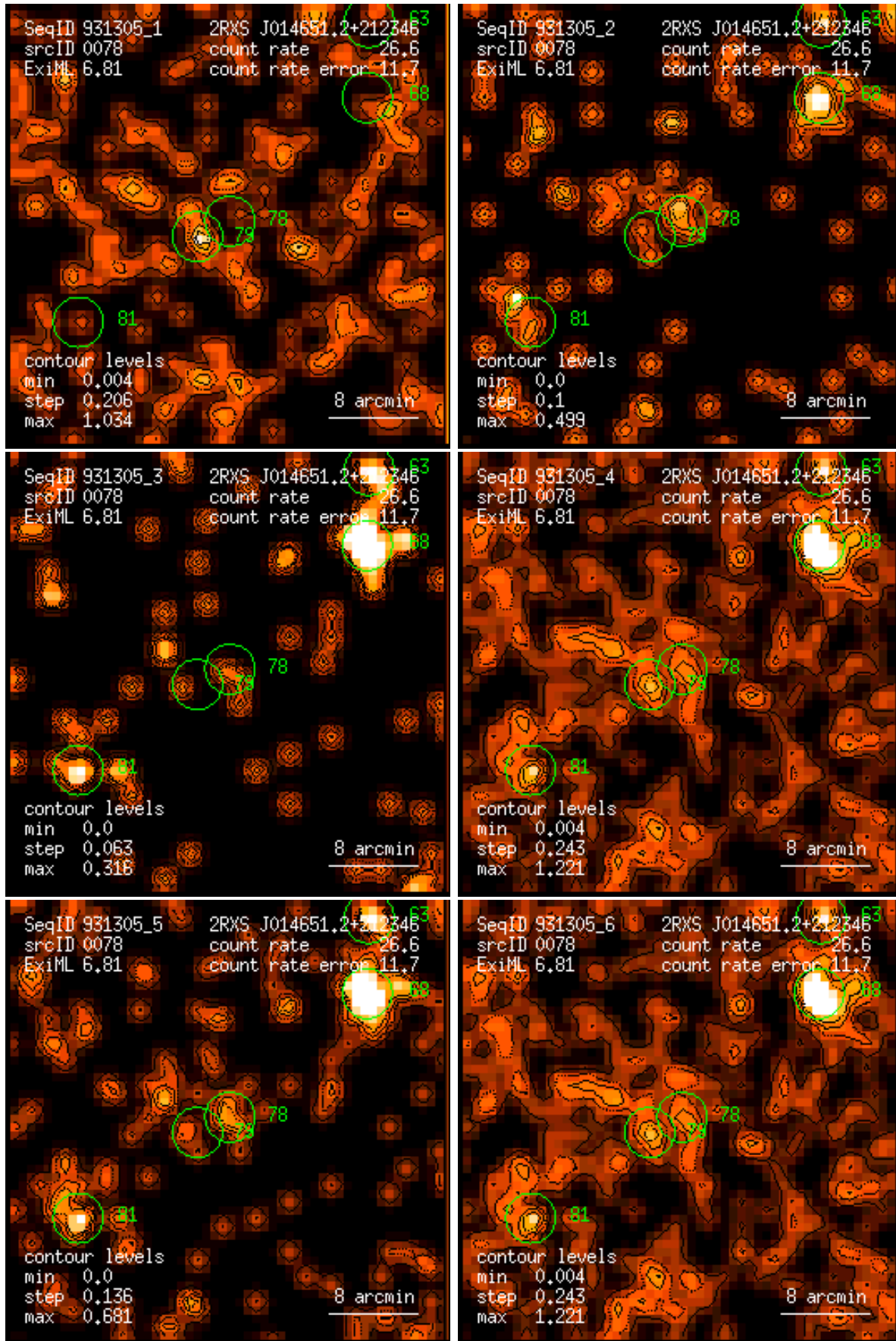
Figure 78: RASS 931305: detection 0078: band rate images, Gaussian filter: (1) PSPC channels 11 – 41, (2) 52 – 90, (3) 91 – 201, (4) 11 – 235, (5) 52 – 201, (6) 11 – 201. Broad band rates in counts/ks. Band rate contour levels in counts/ks/arcmin 2 .
