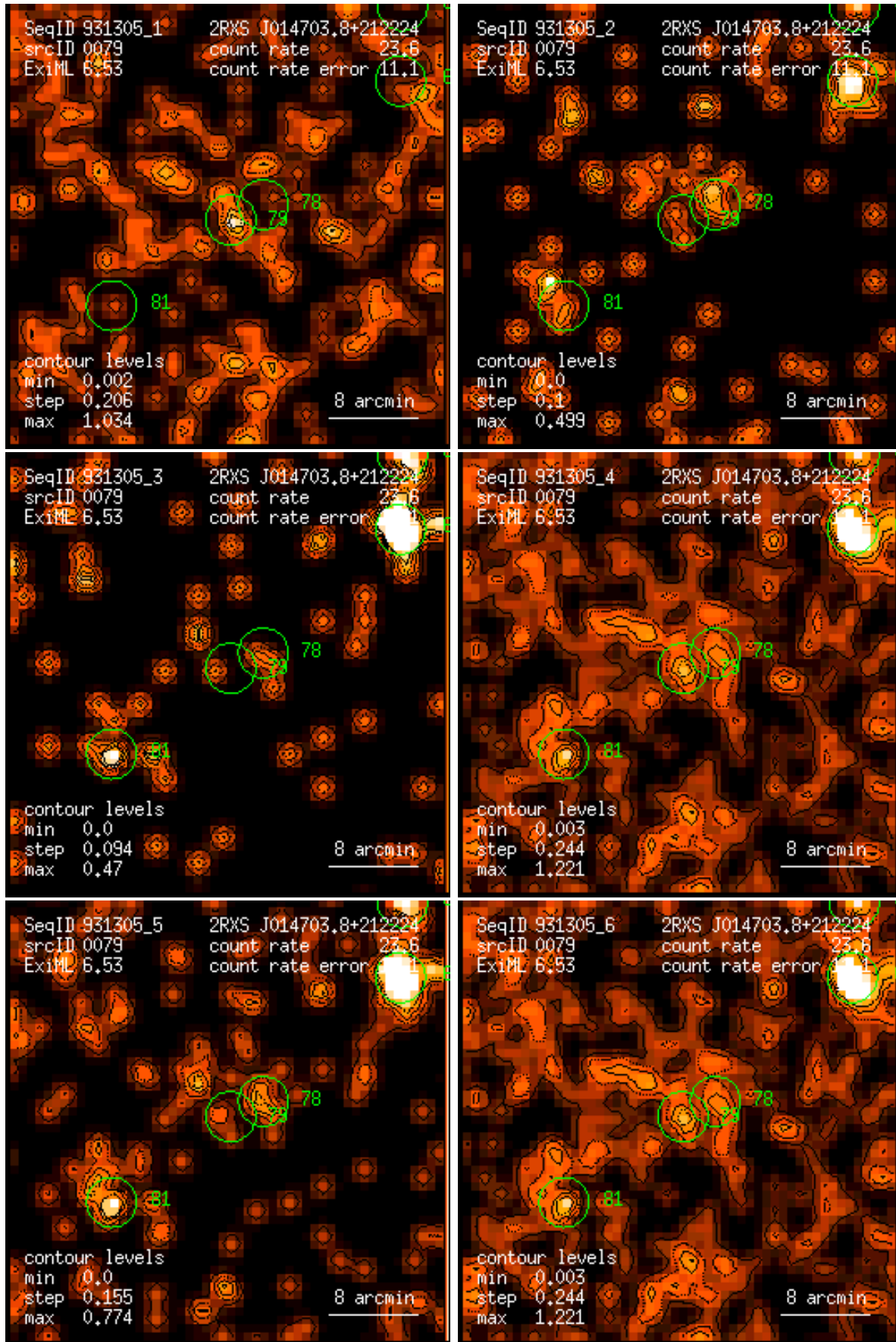
Figure 79: RASS 931305: detection 0079: band rate images, Gaussian filter: (1) PSPC channels 11 – 41, (2) 52 – 90, (3) 91 – 201, (4) 11 – 235, (5) 52 – 201, (6) 11 – 201. Broad band rates in counts/ks. Band rate contour levels in counts/ks/arcmin 2 .
