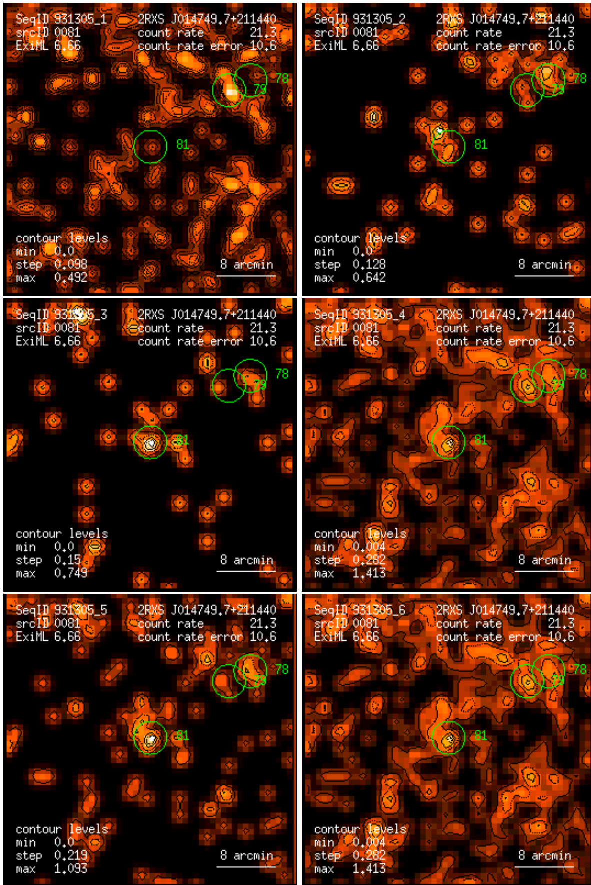
Figure 81: RASS 931305: detection 0081: band rate images, Gaussian filter: (1) PSPC channels 11 – 41, (2) 52 – 90, (3) 91 – 201, (4) 11 – 235, (5) 52 – 201, (6) 11 – 201. Broad band rates in counts/ks. Band rate contour levels in counts/ks/arcmin 2 .
