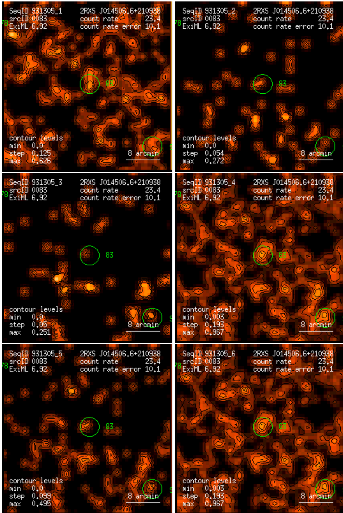
Figure 83: RASS 931305: detection 0083: band rate images, Gaussian filter: (1) PSPC channels 11 – 41, (2) 52 – 90, (3) 91 – 201, (4) 11 – 235, (5) 52 – 201, (6) 11 – 201. Broad band rates in counts/ks. Band rate contour levels in counts/ks/arcmin 2 .
