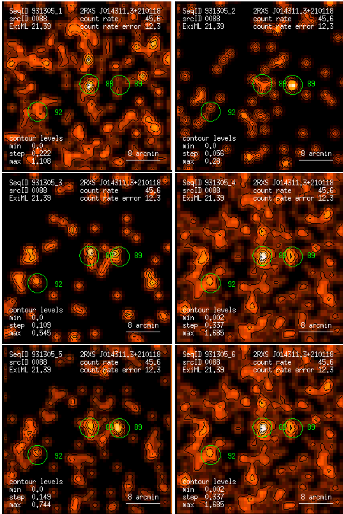
Figure 88: RASS 931305: detection 0088: band rate images, Gaussian filter: (1) PSPC channels 11 – 41, (2) 52 – 90, (3) 91 – 201, (4) 11 – 235, (5) 52 – 201, (6) 11 – 201. Broad band rates in counts/ks. Band rate contour levels in counts/ks/arcmin 2 .
