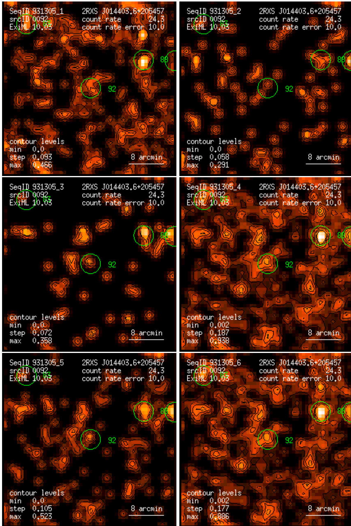
Figure 92: RASS 931305: detection 0092: band rate images, Gaussian filter: (1) PSPC channels 11 – 41, (2) 52 – 90, (3) 91 – 201, (4) 11 – 235, (5) 52 – 201, (6) 11 – 201. Broad band rates in counts/ks. Band rate contour levels in counts/ks/arcmin 2 .
