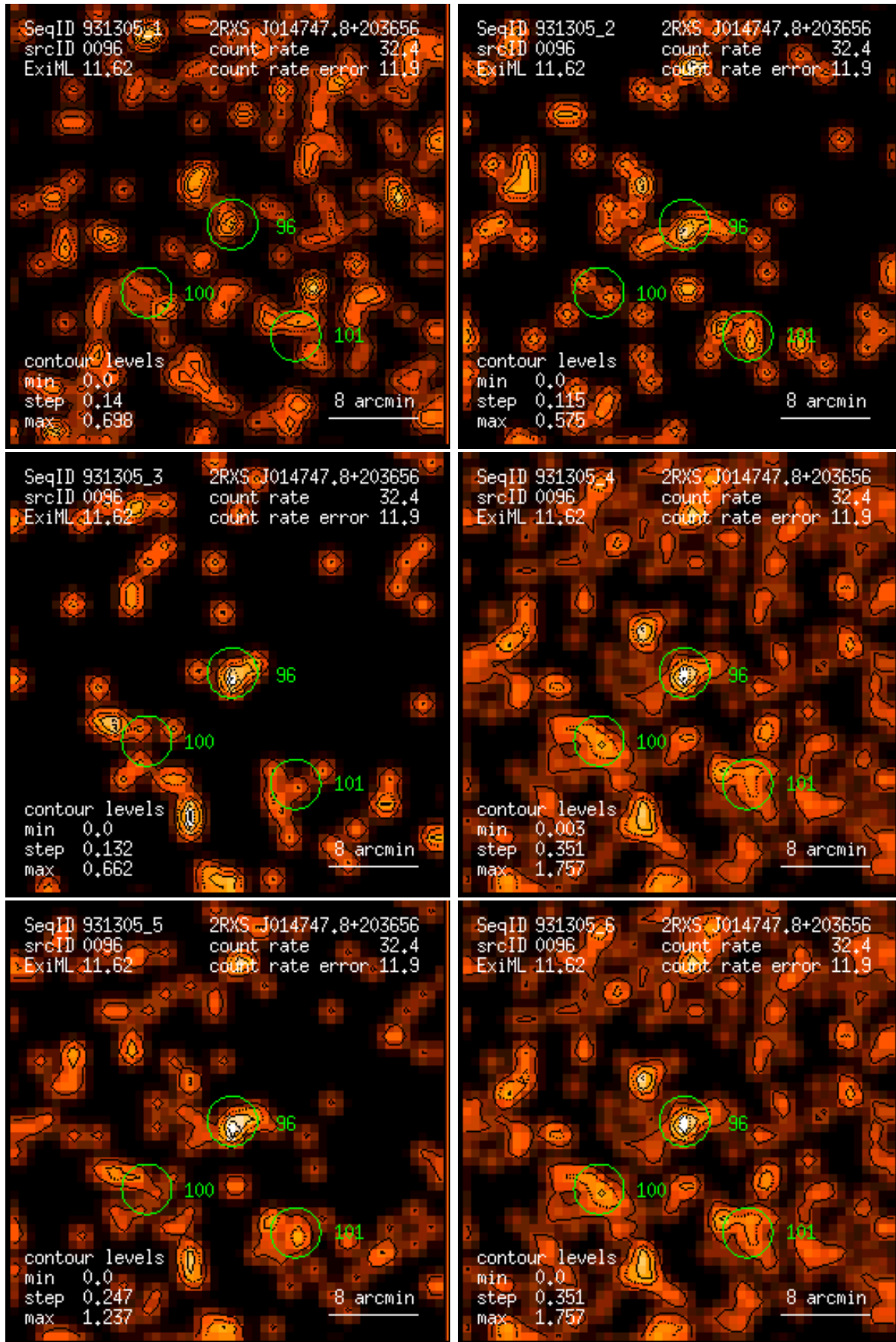
Figure 96: RASS 931305: detection 0096: band rate images, Gaussian filter: (1) PSPC channels 11 – 41, (2) 52 – 90, (3) 91 – 201, (4) 11 – 235, (5) 52 – 201, (6) 11 – 201. Broad band rates in counts/ks. Band rate contour levels in counts/ks/arcmin 2 .
