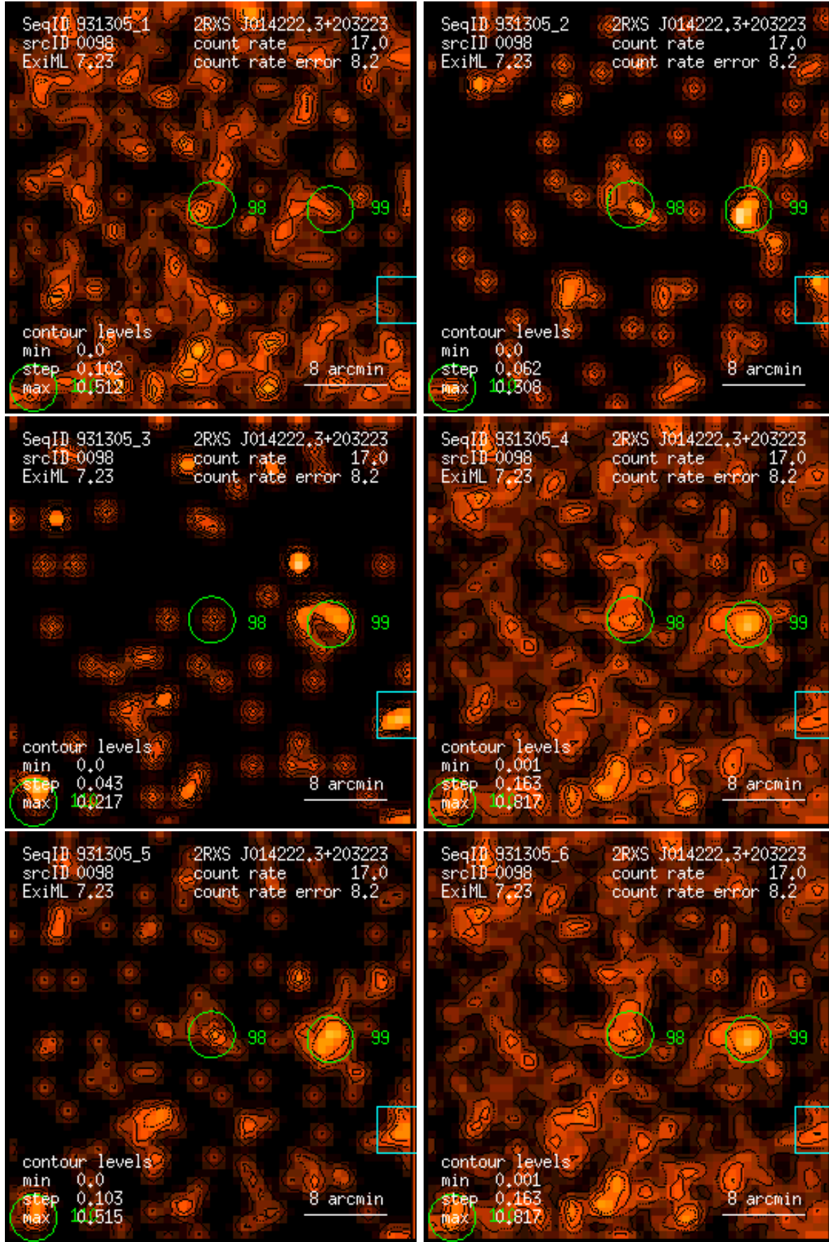
Figure 98: RASS 931305: detection 0098: band rate images, Gaussian filter: (1) PSPC channels 11 – 41, (2) 52 – 90, (3) 91 – 201, (4) 11 – 235, (5) 52 – 201, (6) 11 – 201. Broad band rates in counts/ks. Band rate contour levels in counts/ks/arcmin 2 .
