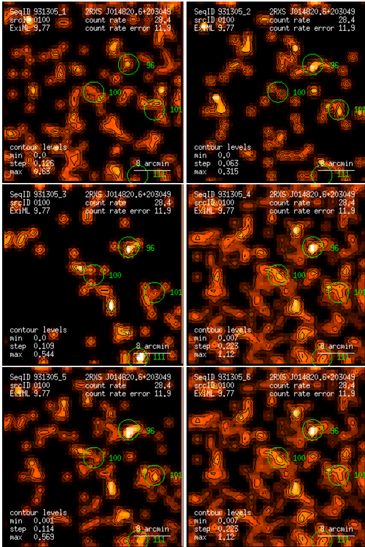
Figure 100: RASS 931305: detection 0100: band rate images, Gaussian filter: (1) PSPC channels 11 – 41, (2) 52 – 90, (3) 91 – 201, (4) 11 – 235, (5) 52 – 201, (6) 11 – 201. Broad band rates in counts/ks. Band rate contour levels in counts/ks/arcmin 2 .
